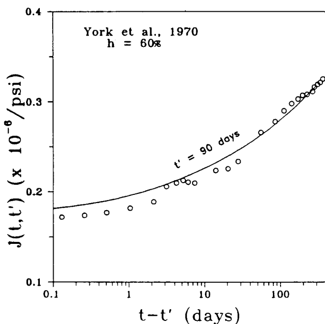
Fig. 4 Predictions of drying creep and data by York et al. [19].
