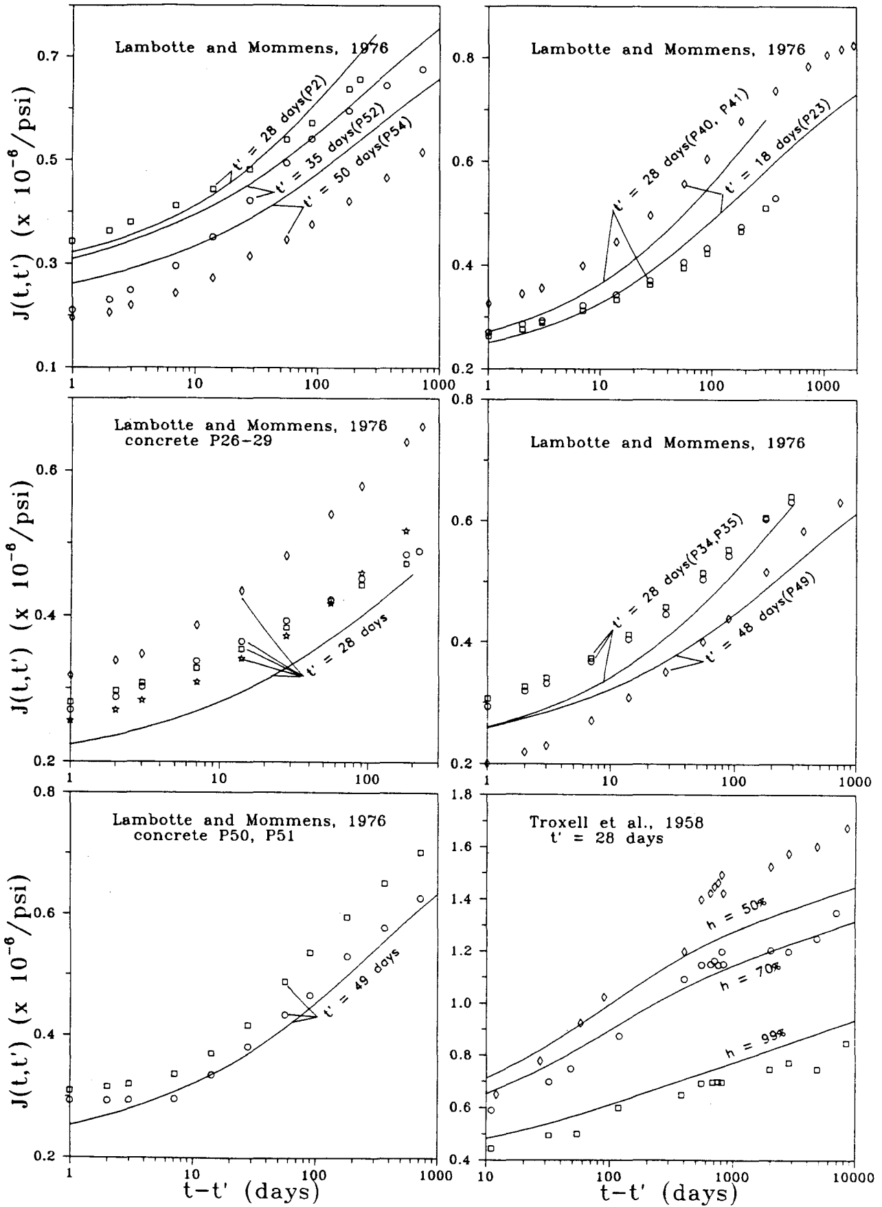
Fig. 2 Predictions of drying creep and data by Lambotte and Mommens [11] and Troxell et al. [18].
