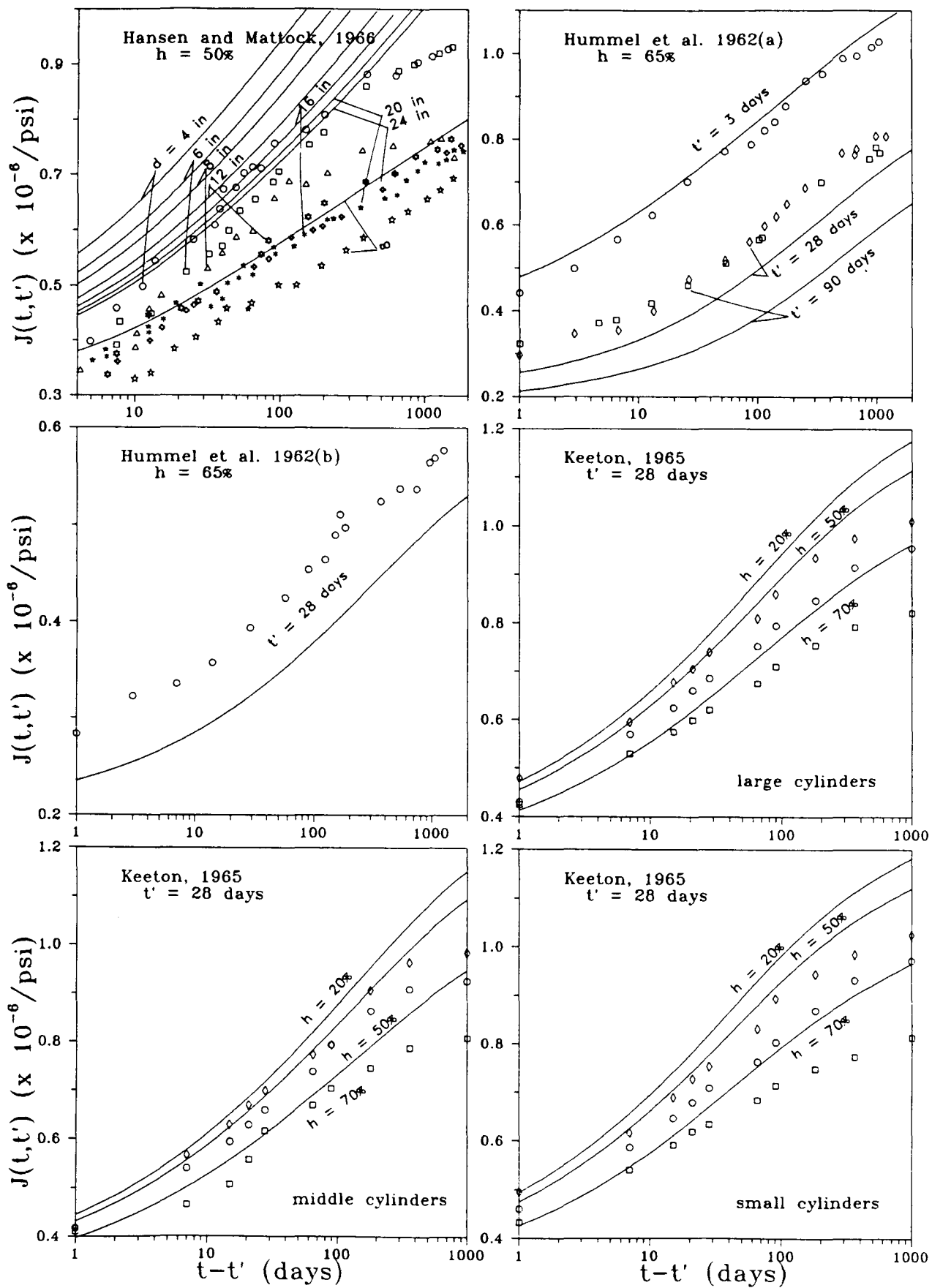
Fig. 1 Predictions of drying creep and data by Hansen and Mattock [8], Hummel et al. [9] and Keeton [10].
