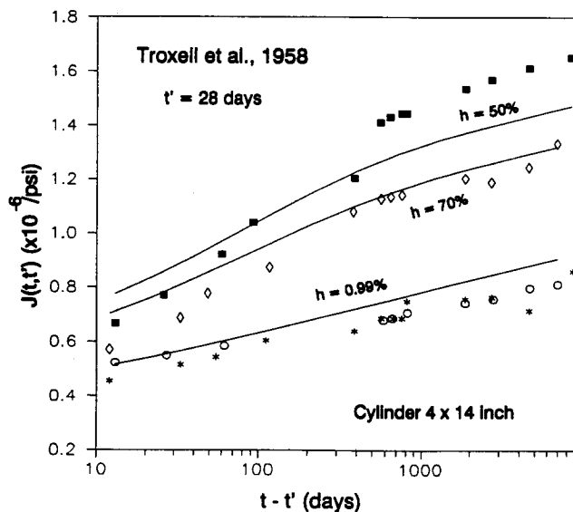
Fig. 6 Predictions of drying creep data by Troxell et al. [11] (1 psi = 6895 Pa).
