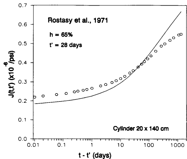
Fig. 5 Prediction of drying creep data by Rostasy et al. [10] (1 psi = 6895 Pa).
