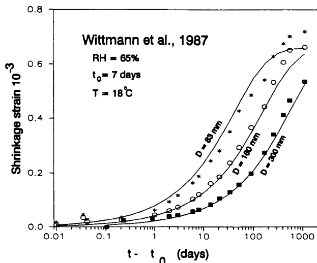
Fig. 2 Predictions of shrinkage data by Wittmann et al. [7].
