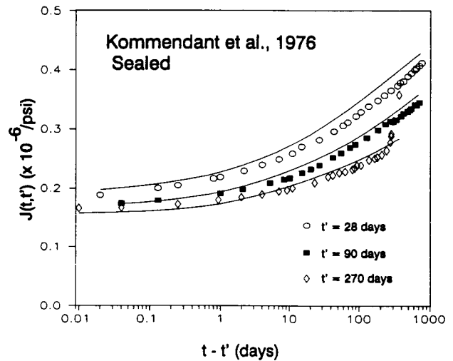
Fig. 4 Predictions of basic creep test by Kommendant et al. [9] (1 psi = 6895 Pa).
