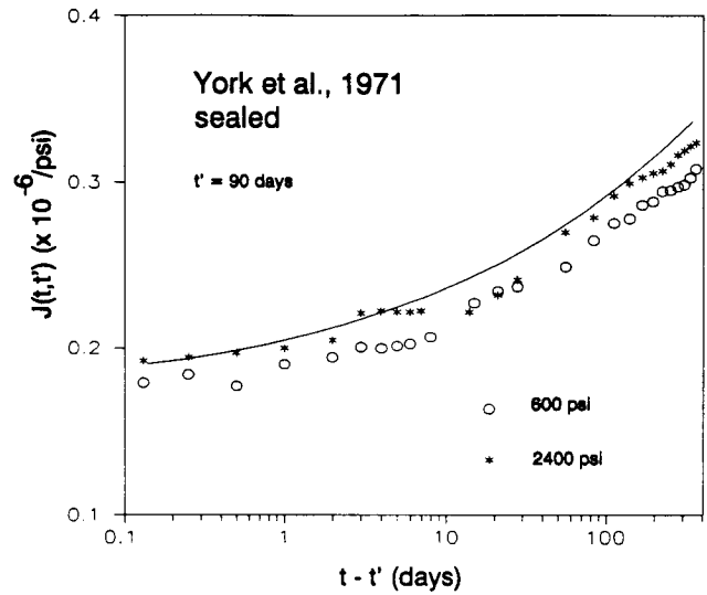
Fig. 3 Predictions of basic creep data by York et al. [8] (1 psi = 6895 Pa).
