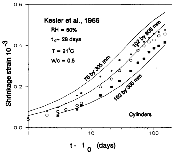
Fig. 1 Predictions of shrinkage test data by Kesler et al. [6].
