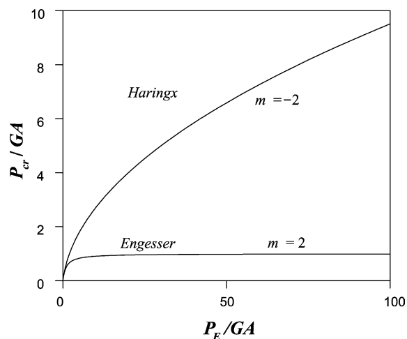
Fig. 1. Difference between the Engesser-type and Haringx-type formulae for a sandwich with E_{\text{skin}}/G_{\text{core}} \approx 1400 .
