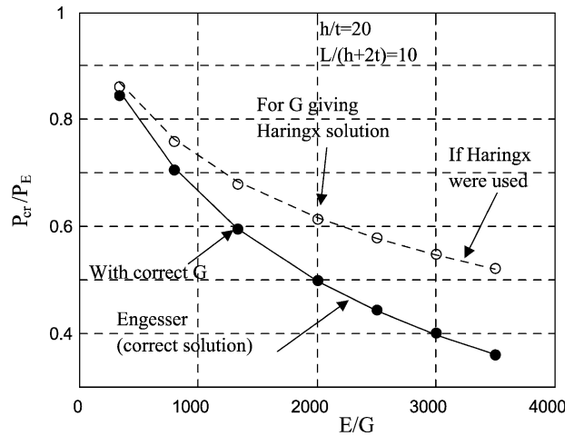
Fig. 10. Critical load for short column with thin skin and stiff plate at the top.
