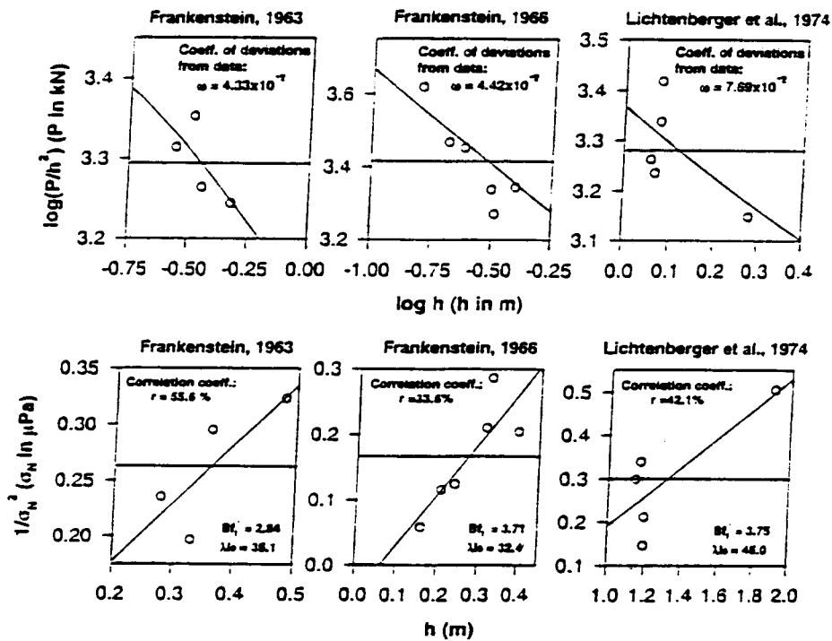
Figure 1. Size effect plots of existing test data (Frankenstein 1963, 1966; Lichtenberger et al. 1974) in terms of nominal strength \sigma_N .
