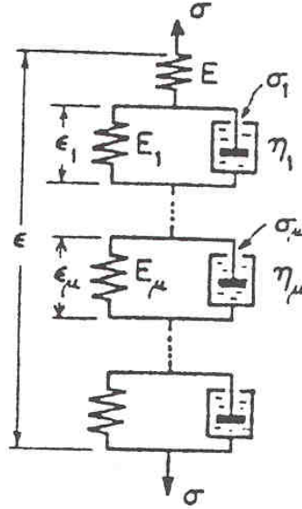
Figure 4: Kelvin chain model with age-dependent spring moduli E_\mu(t) and viscosities \eta_\mu(t) .
