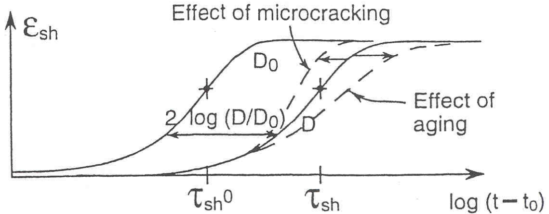
Figure 12: Shrinkage curve viewed as interpolation between theoretically determined asymptotic behaviors for short and long drying times.
