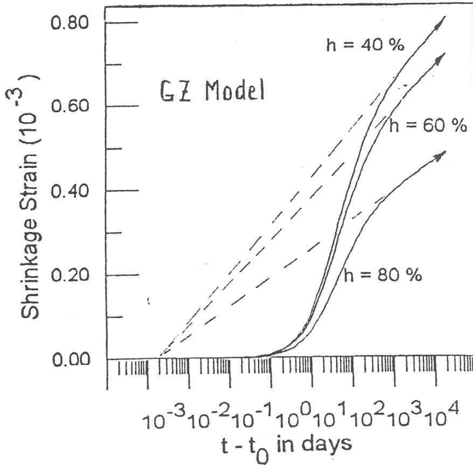
Figure 10: Typical shrinkage curves of GZ model ( h = environmental humidity).
