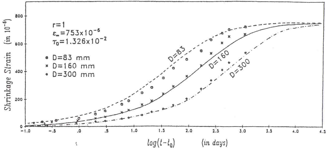
Figure 13: Shrinkage measured by Wittmann et al. (1997) (data points) compared to curves for which the halftimes are scaled as the square of diameter of the cylinder, as required by diffusion theory.
