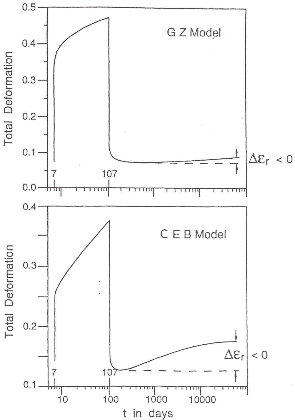
Figure 6: Unrealistic recovery reversal obtained by principle of superposition for GZ and CEB-FIP models.
