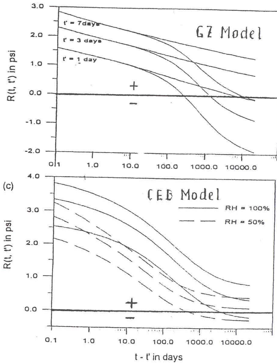
Figure 7: Unrealistic change of sign of relaxation curves obtained according to the principle of superposition. Strain 10^{-6} applied at age t' . R.H. = 100% upper branches, 50% lower branches ( t_0 = 1 day). GZ model: f'_c = 50 MPa, CEB-FIP model: f'_c = 35 MPa.
