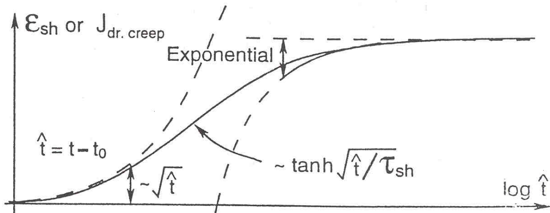
Figure 14: According to diffusion theory, a change of diameter from D_0 to D causes a horizontal shift by distance 2 \log(D/D_0) . The effects of cracking and aging distort it but in opposite ways.
