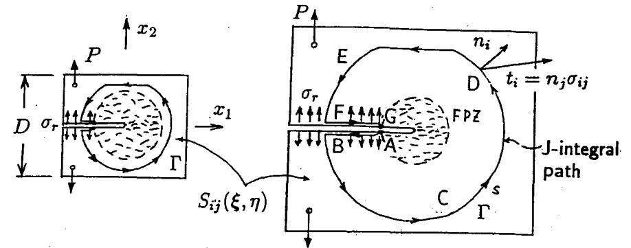
Fig. 1 Path of J-integral for size effect analysis
