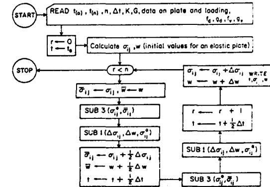
Fig. 4. Flow chart of the second-order method in the case of rate-type creep ( n = subdivision of time; T = true, F = false).
