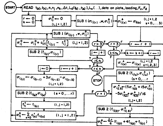
FIG. 1. Flow chart of the fourth-order method in the case of integral-type creep, valid for n \geq 3 ( n = subdivision of time; n_1 = number of iterations; n_k = number of approximations; T = true, F = false; SUB1, SUB2 = subroutines defined in the text).
