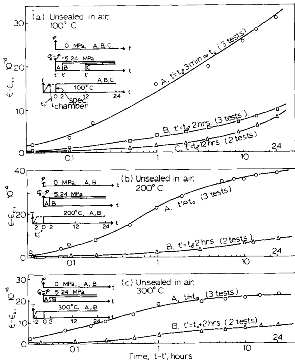
Fig. 6. — Effect of Preheating Period on Creep of Unsealed Specimens in Air.
