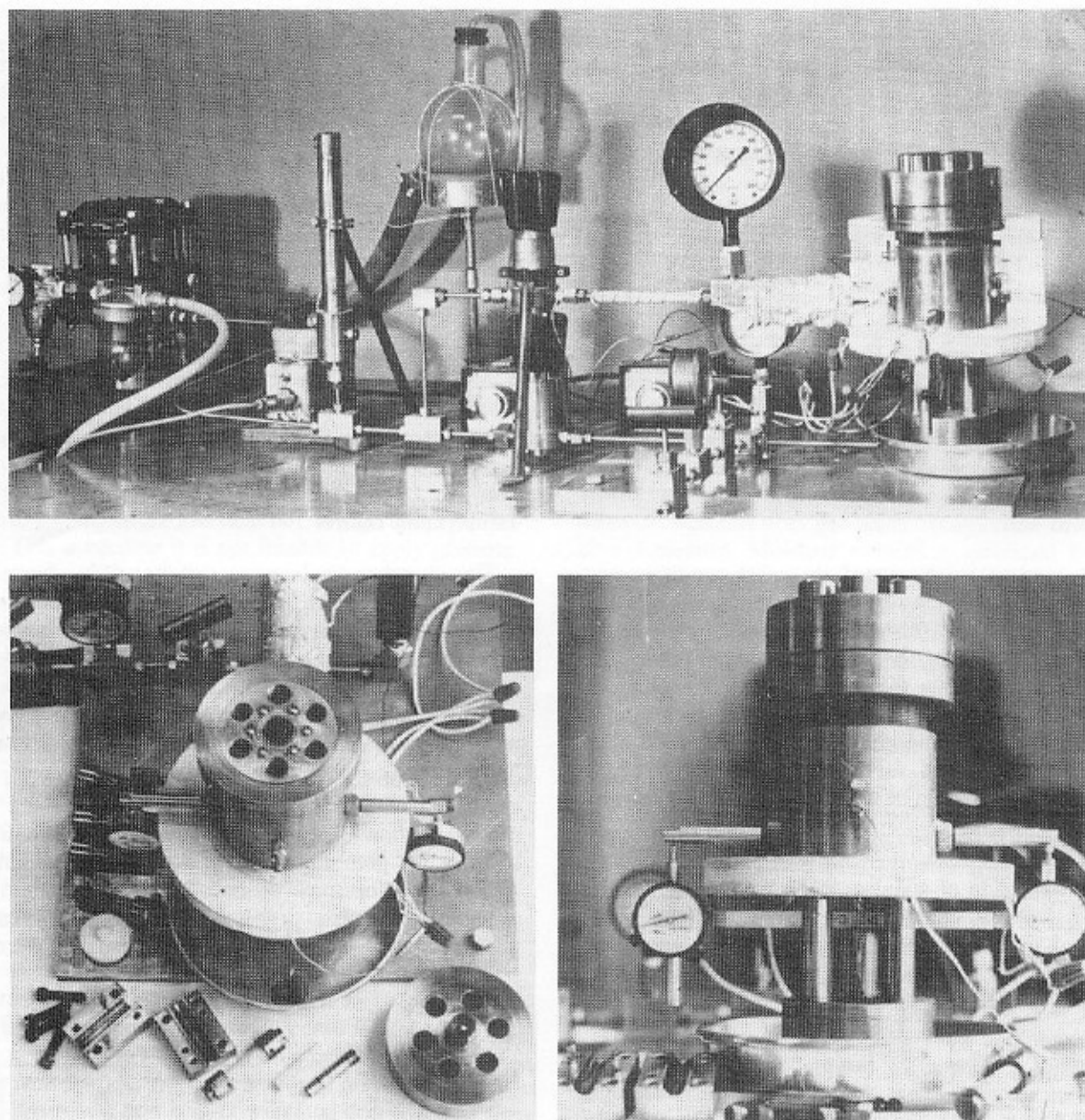
Fig. 3. — Photographs of the Test Specimen, Chamber, and Test Set-Up.
