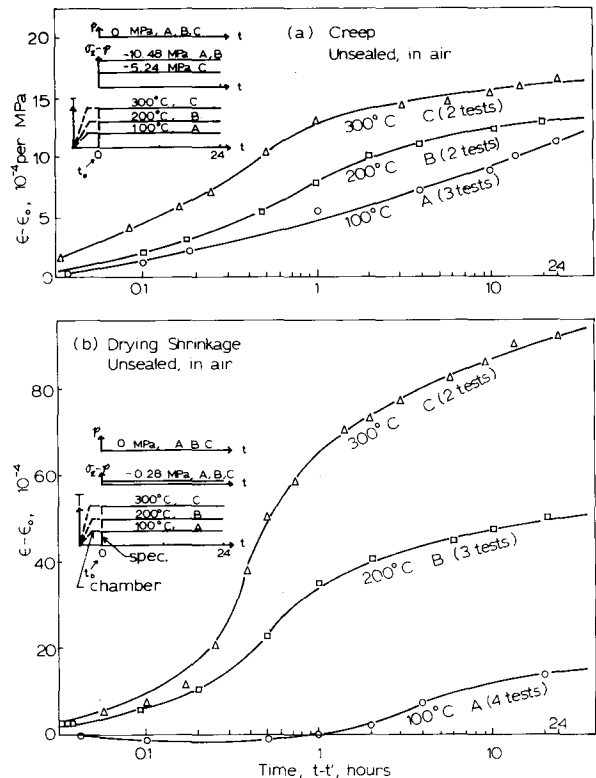
Fig. 8. — Effect of Temperature on Drying Creep and Shrinkage.
