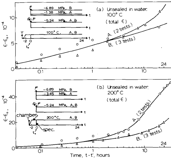
Fig. 7. — Effect of Pressure on Creep of Unsealed Specimens in Water at Various Temperatures.
