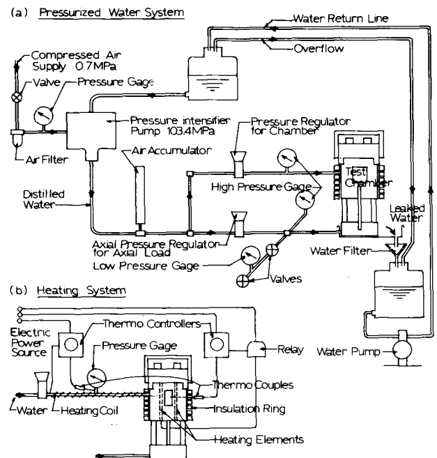
Fig. 2. — Pressurization and Heating Systems Used.
