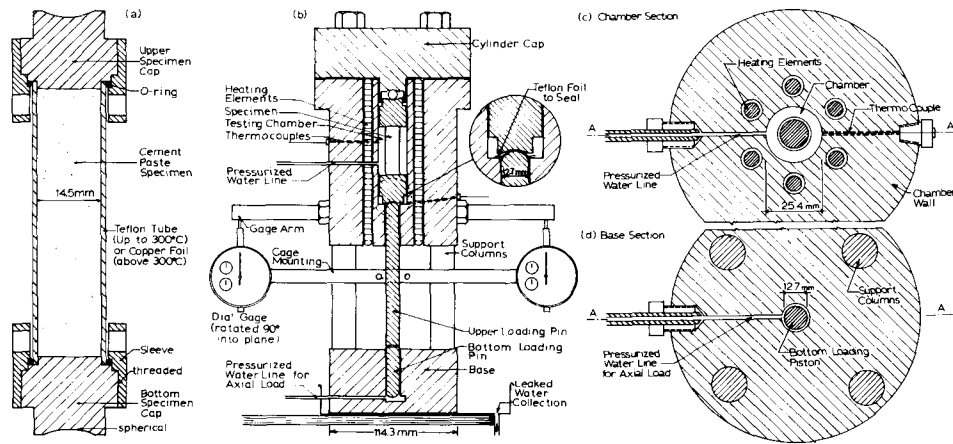
Fig. 1. — Cross Sections of Test Specimen (a) and of Heated Triaxial Test Chamber (b), and Horizontal Sections of the Chamber (c, d).
