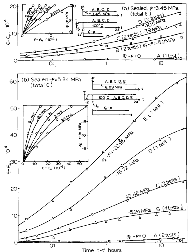
Fig. 5. — Axial Creep of Sealed Specimens at Various Axial Stresses and Pressures.
