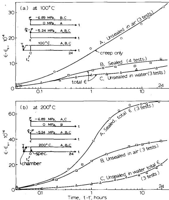
Fig. 4. — Comparison of Creep of Sealed Specimens and Unsealed Specimens in Air or Water.
