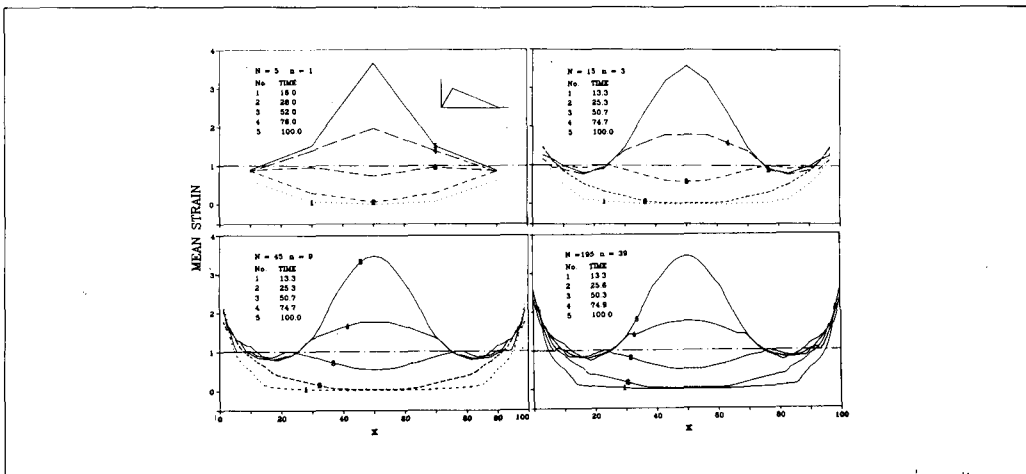
Fig. 5. Numerical Results of Bazant, Chang, and Beltyshko [1] for Wave Propagation in a Strain-Softening Bar.
