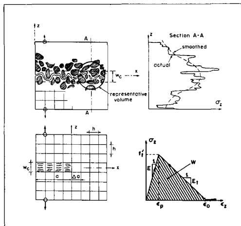
Fig. 1. Fracture in a Heterogeneous Material; Statistical Scatter of Stresses, Crack Band Model, and Strain-Softening Stress-Strain Diagram.
