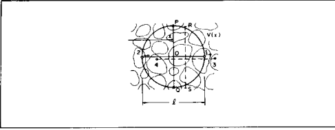
Fig. 2. Characteristic Volume of a Heterogeneous Material (the broad range stress at point 0 depends on the relative displacements at Points 1 and 2 but not on those at Points 3 and 4).
