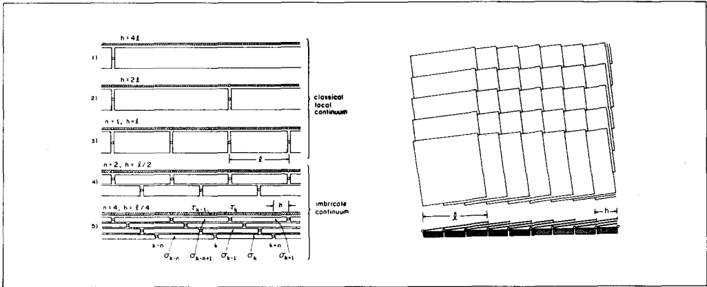
Fig. 4. Illustration of Mesh Refinement for a One-Dimensional Imbricate Continuum, and of Element Arrangement for a Two-Dimensional Imbricate Continuum (the elements are slightly rotated for the purpose of illustration).
