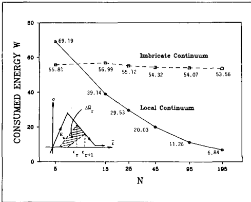
Fig. 6. Energy Consumed by Failure Caused by Wave Propagation in a One-Dimensional Bar.
