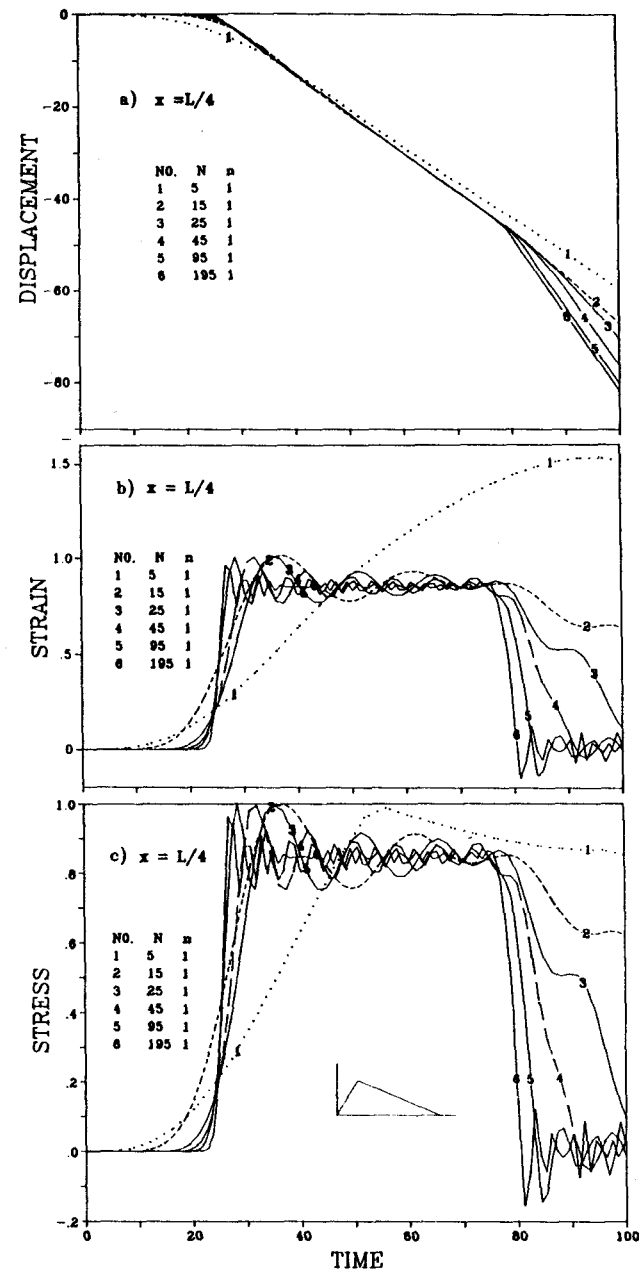
FIG. 3.—Results for Strain-Softening Local Continuum—Convergence of Time History
