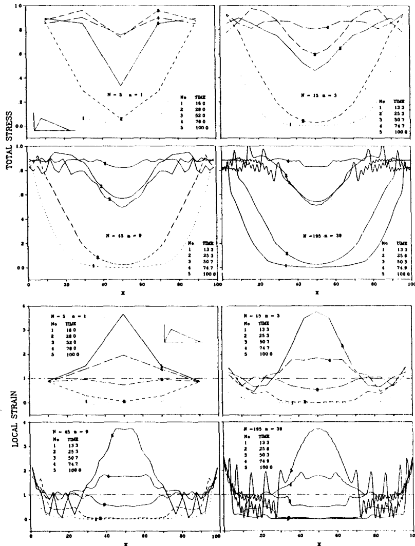
FIG. 9.—Fully Strain-Softening Imbricate Continuum—Further Results on Convergence of Spatial Distributions with Mesh Refinement
