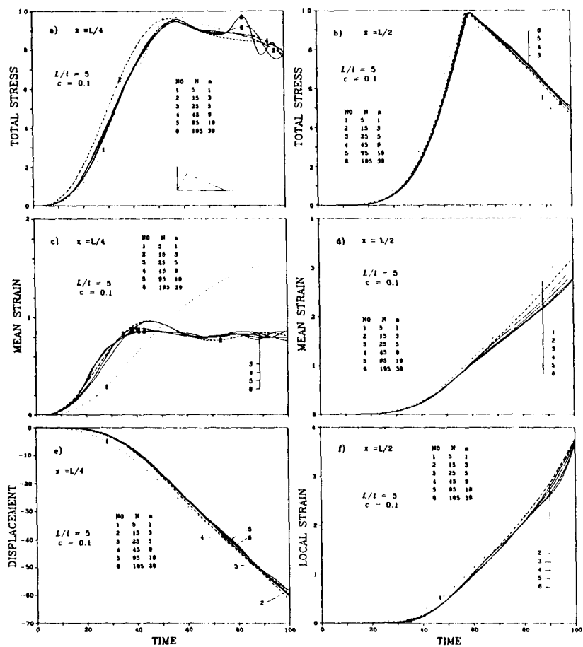
FIG. 7.—Results for Fully Strain-Softening Imbricate Continuum—Convergence of Time Histories at Mesh Refinement
