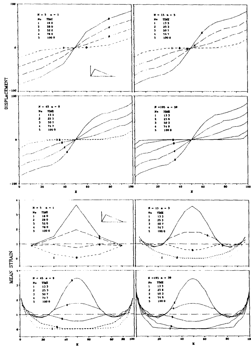
FIG. 8.—Results for Fully Strain-Softening Imbricate Continuum—Convergence of Spatial Distributions at Various Times with Mesh Refinement
