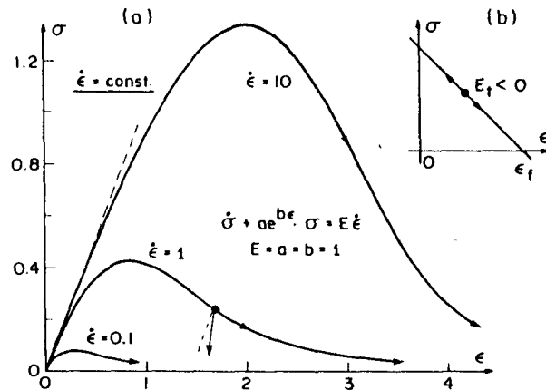
FIG. 1.—Inadequate Models for Strain-Softening: (a) Rate Effect; (b) Linear Material of Negative Modulus
