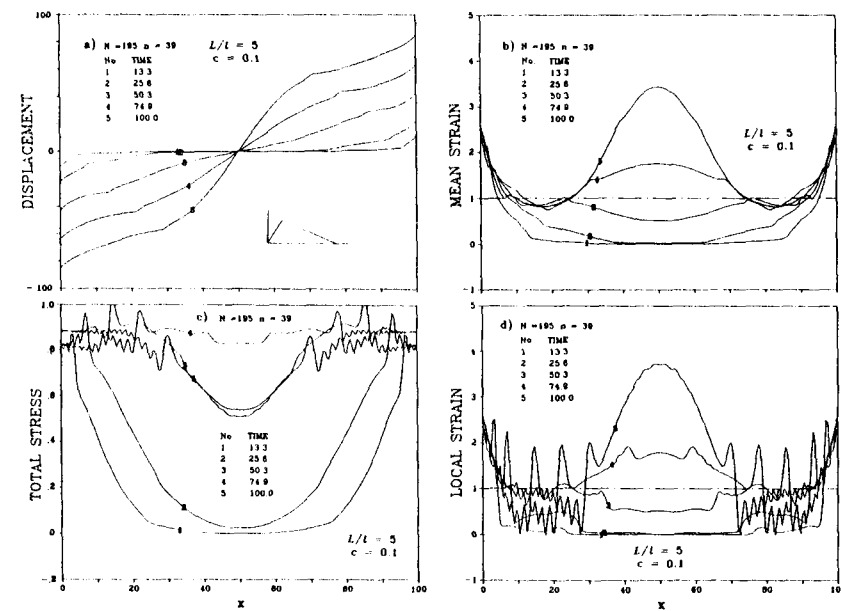
FIG. 6.—Results for Fully Strain-Softening Imbricate Continuum, for Finest Mesh
