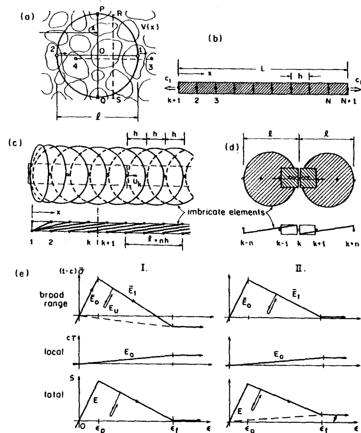
FIG. 2.—Imbricate Nonlocal Continuum: (a) Representative Volume; (b–d) System of Local and Imbricate Elements; (e) Stress-Strain Diagrams
