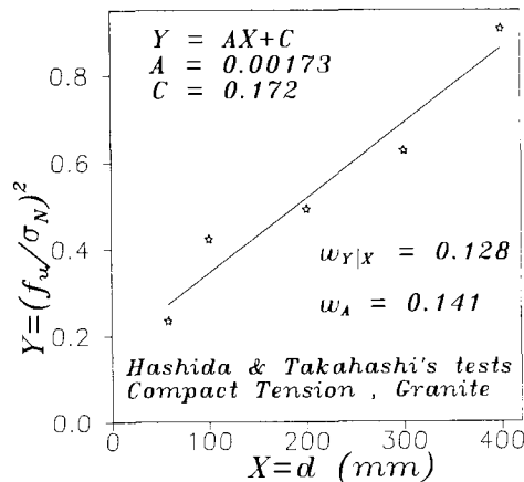
Fig. 2. Linear regression plot for granite, compact tension specimens with average α 0 = 0.544.
