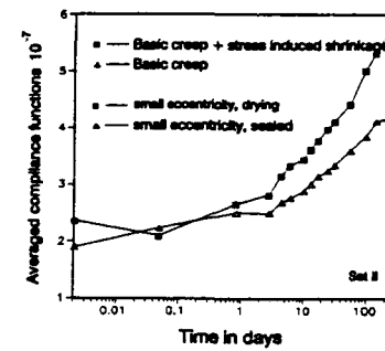
Fig. 8 Averaged compliance functions
