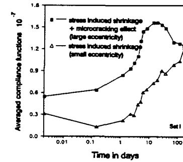
Fig. 6 Decomposition of different drying creep mechanisms
