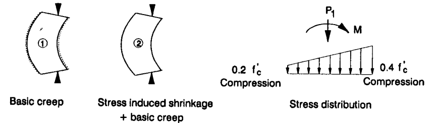
Fig. 2 Experimental plan I: small eccentricity
