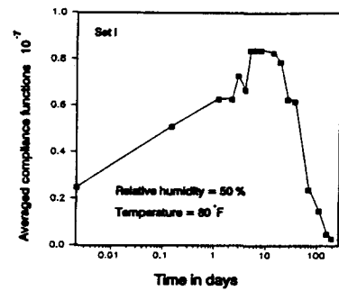
Fig. 7 Effect of microcracking on drying creep
