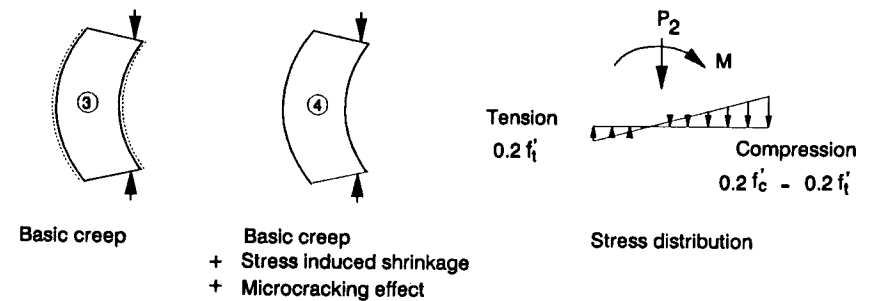
Fig. 3 Experimental plan II: large eccentricity
