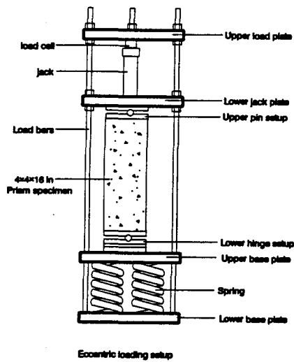
Fig. 4 Experiment setup
