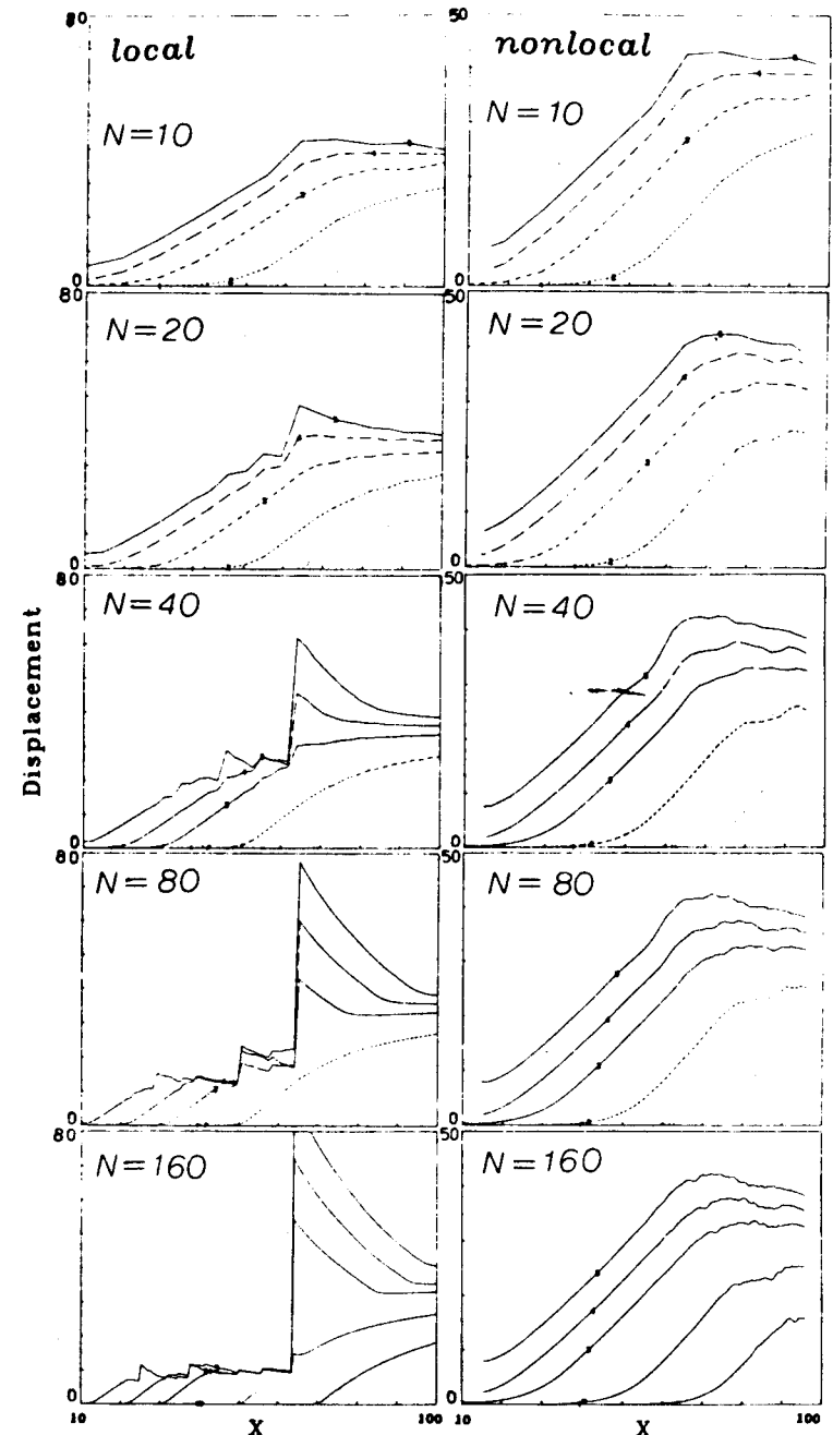
Figure 7. Radial displacement profiles at various times obtained for various finite element subdivisions ( N = \text{number of elements} )
