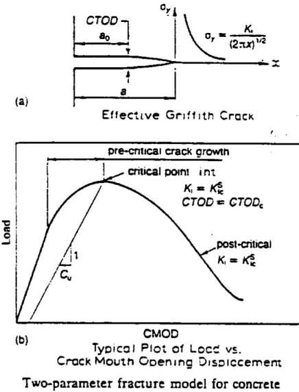
Fig.4.1 Two Parameter Fracture Model of Jenq and Shah (1985)
