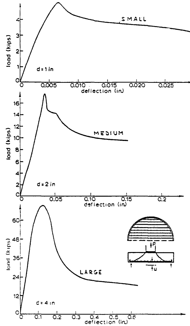
Fig.1.12 Measured Load-Deflection Diagrams of Small, Medium and Large Slabs (Bažant and Cao, 1987)
