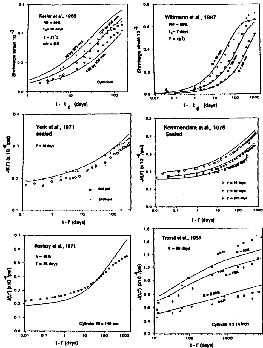
Fig. 1 Examples of Comparison of Simplified BP-KX Model with Test Data by Kesler et al. (top left), Wittmann et al. (top right), York et al. (middle left), Kommedant et al. (middle right), Rostasy et al. (bottom left) and Troxell et al. (bottom right); after Part 6 of Bazant, Kim and Xi, 1992.
