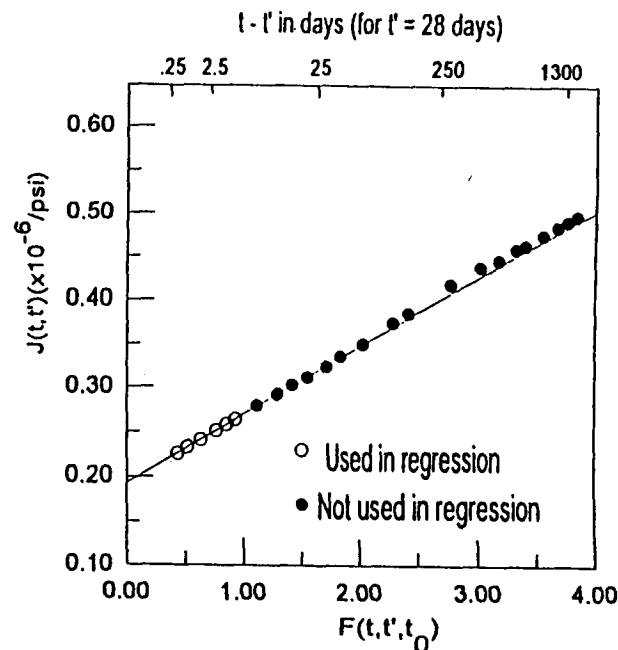
Fig. 3 Example of Updating the Model Parameters by Means of Regression of Short-Time Measurements of Creep.
