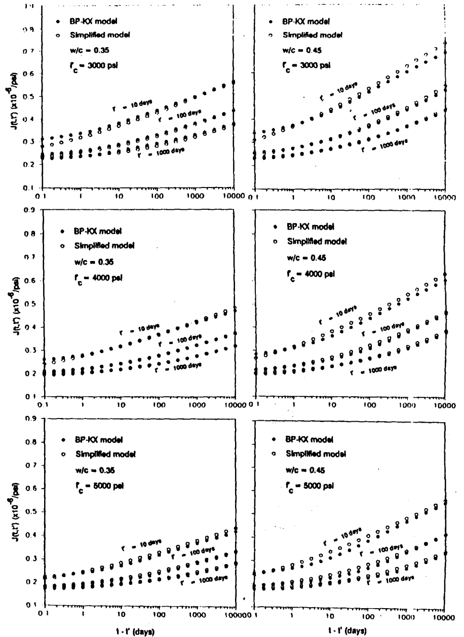
Fig. 2 Comparisons of the Simplified and Full BP-KX Models for w/c = 0.35 (left) and w/c = 0.45 (right).
