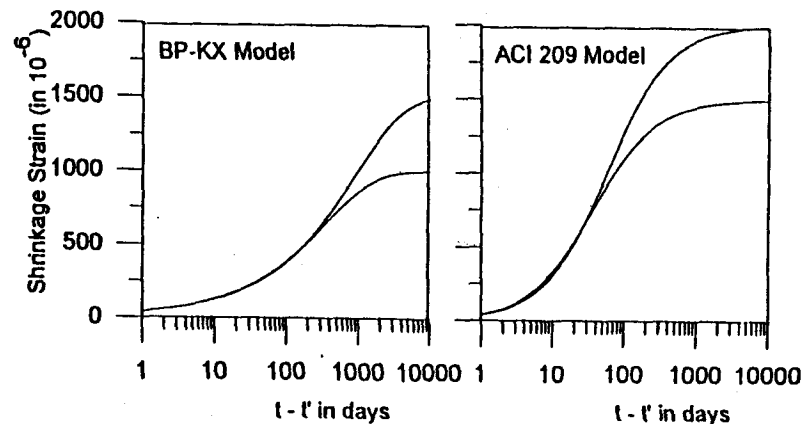
Fig. 4 Example of Shrinkage Curves Giving Nearly the Same Initial Shrinkage but Very Different Final Values (left : \epsilon = 1500 \tanh(i/1500)^{1/2} and 1000 \tanh(i/600)^{1/2} ; and right : \epsilon = 2000i/(55 + i) and 1500i/(35 + i) ).
