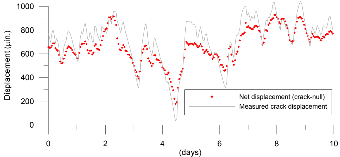
Figure 3.11 Comparison of net displacement and actual measured crack displacement in the field application of the out-of-plane measuring system
