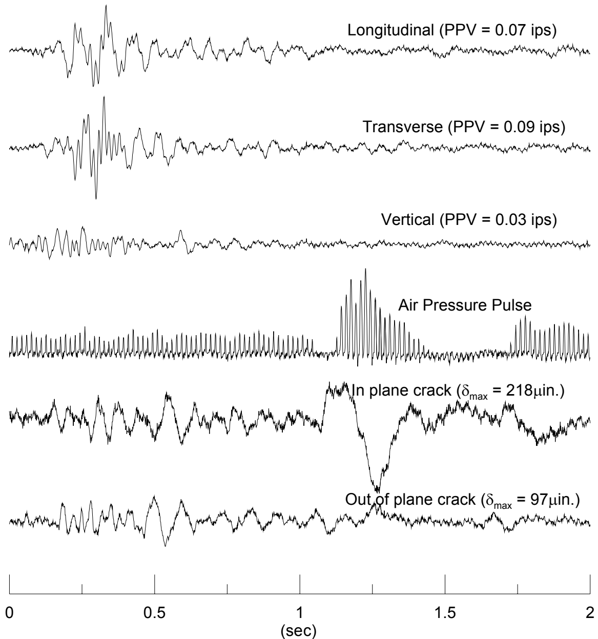
Figure 3.12 Ground motions and associated crack displacements for December 15 th blast
