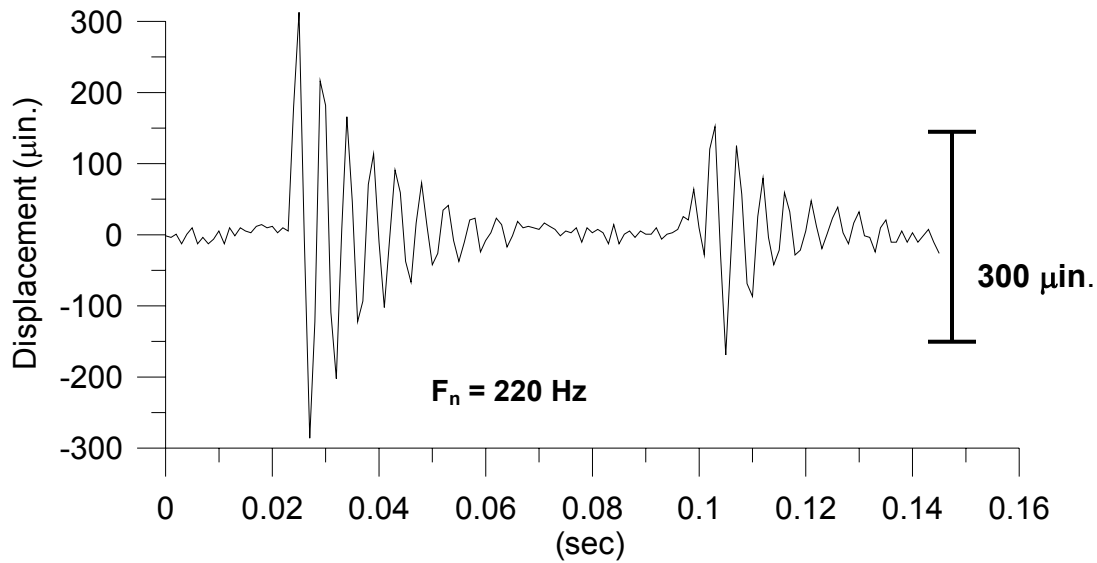
Figure 3.5 Dynamic testing of the out-of-plane displacement measuring system
