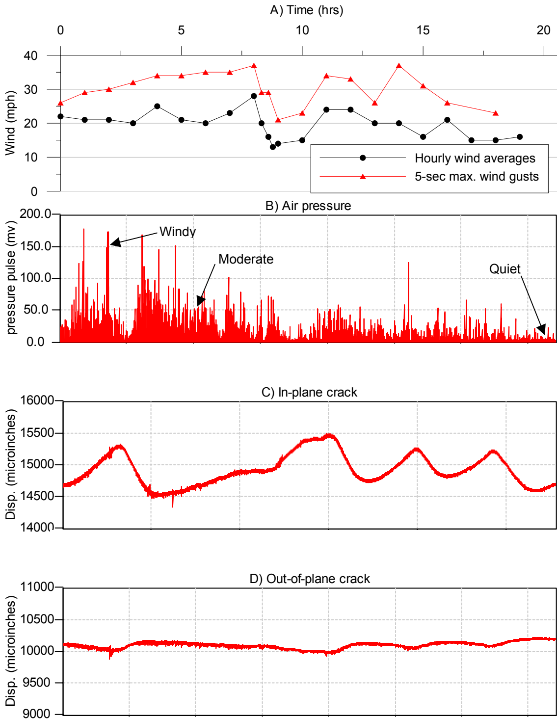
Figure 3.16 Comparison of 20 hours wind and air pressure data vs. crack displacement a) Milwaukee airport wind data b) air pressure data obtained at site c) in-plane crack displacement d) out-of-plane crack displacement
