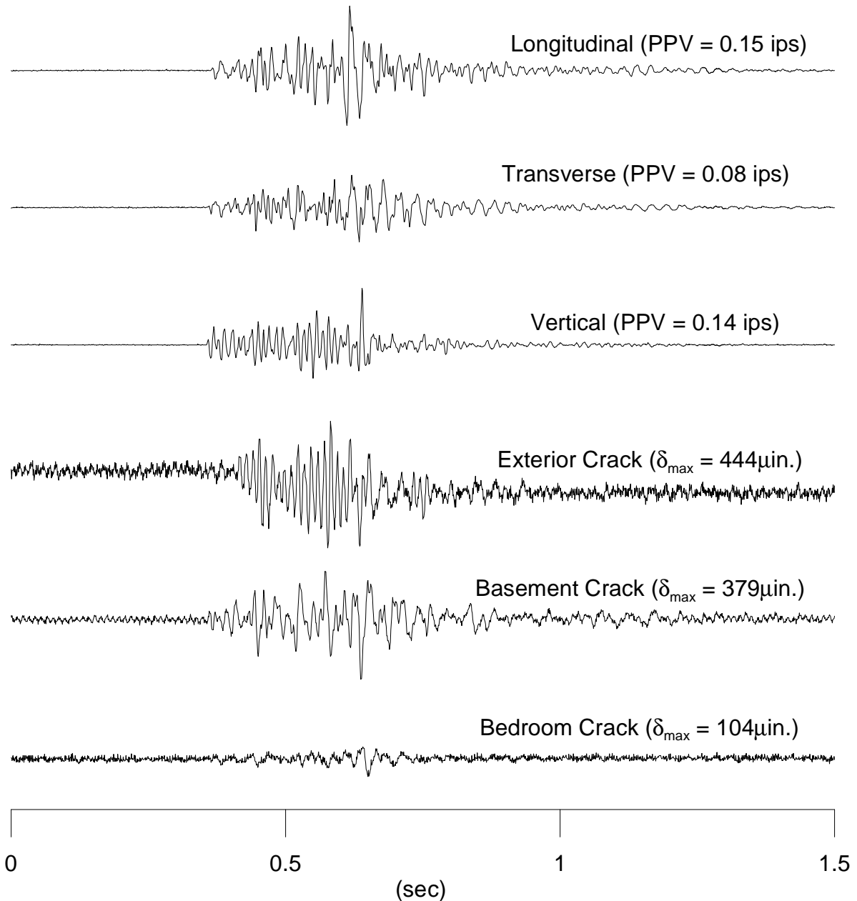
Figure 2.22 Ground motions and crack response for Comp the January 20 th blast
