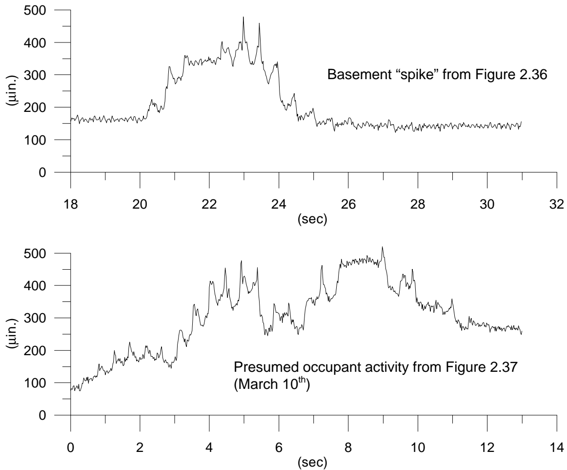
Figure 2.38 Comparison of basement and bedroom spikes seen during 50 Hz testing
