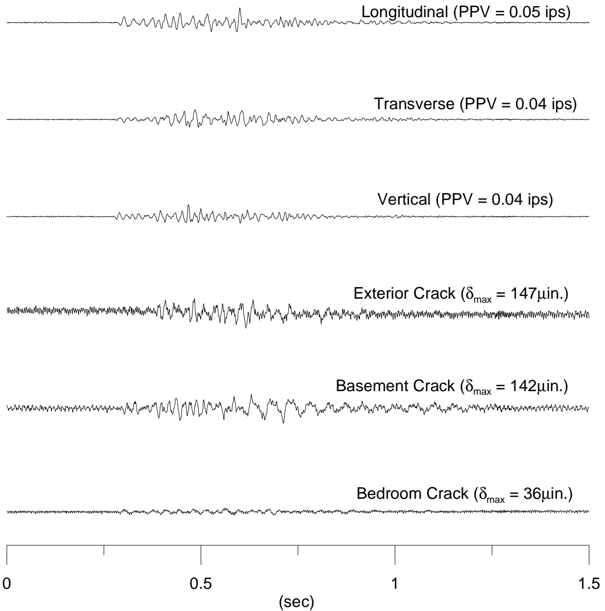
Figure 2.24 Ground motions and crack response for the May 17 th blast
