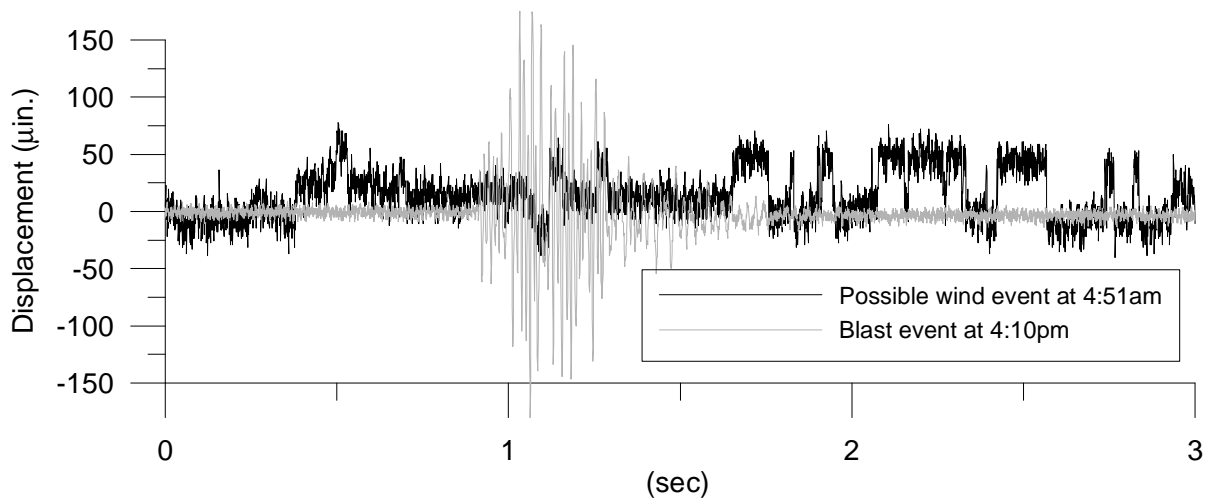
Figure 2.44 Exterior crack displacement due to unknown event recorded during electrical noise spike and a blast event (February 16 th , 2005)
