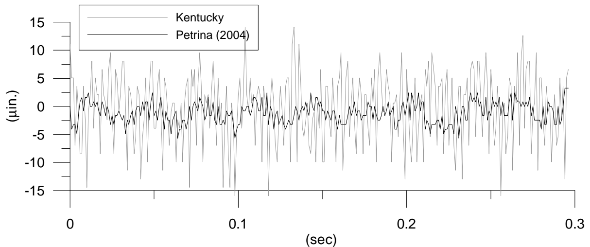
Figure 2.43 Comparison of noise levels for different ACM systems. Shielded CAT5 cables were employed in Kentucky while Petrina utilized instrumentation cable
