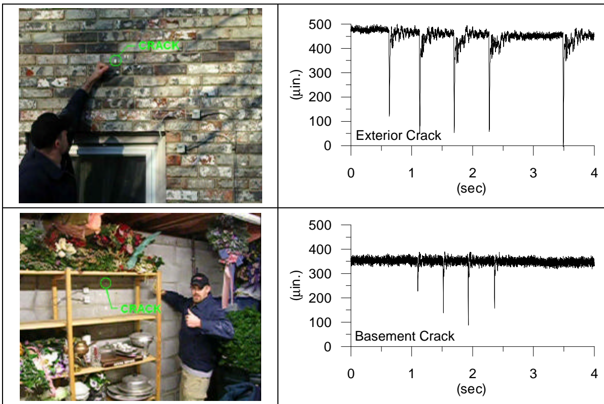
Figure 2.32 Induced occupant activity for exterior and basement cracks
