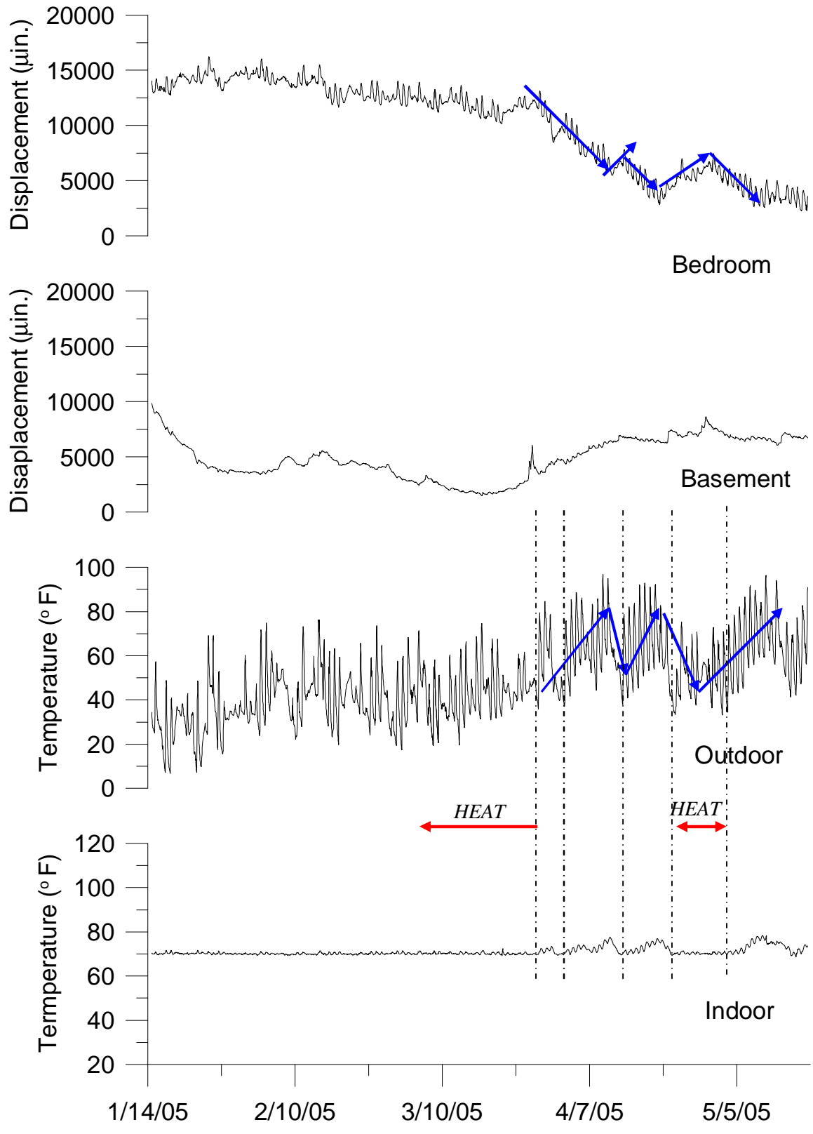
Figure 2.13 Interior crack displacements compared to both indoor and outdoor temperature changes
