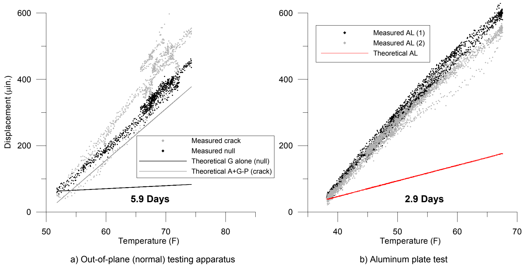
Figure 3.7 Hysteresis loops for out-of-plane (normal) system laboratory qualification tests a) two sensors mounted on glass block; null measures glass response only; crack measures difference between plastic, aluminum, and glass as shown in Figure 3.4 b) two sensors mounted on aluminum plate
