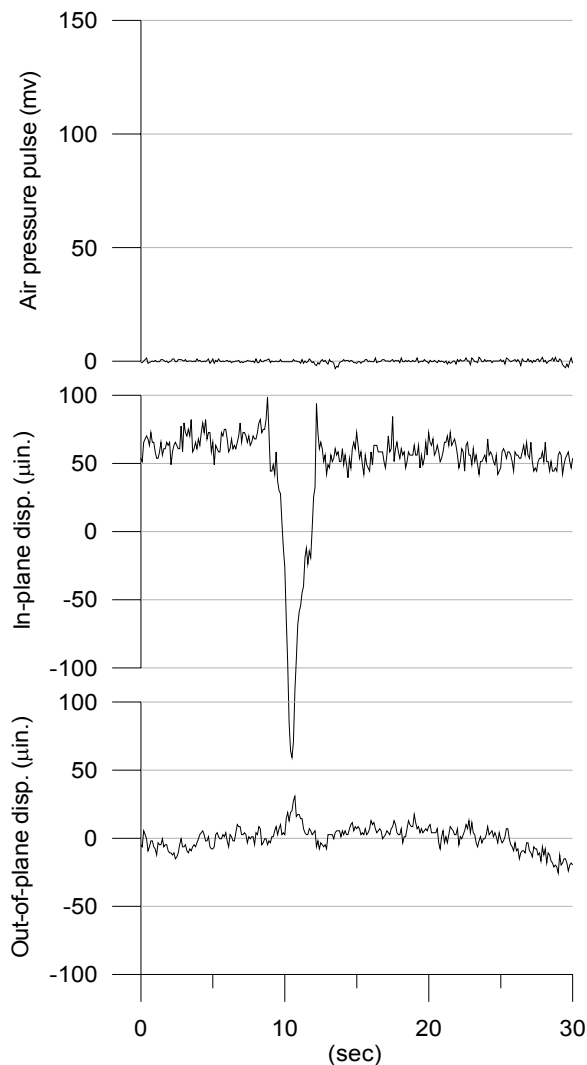
Figure 3.18 Crack behavior when no wind present
