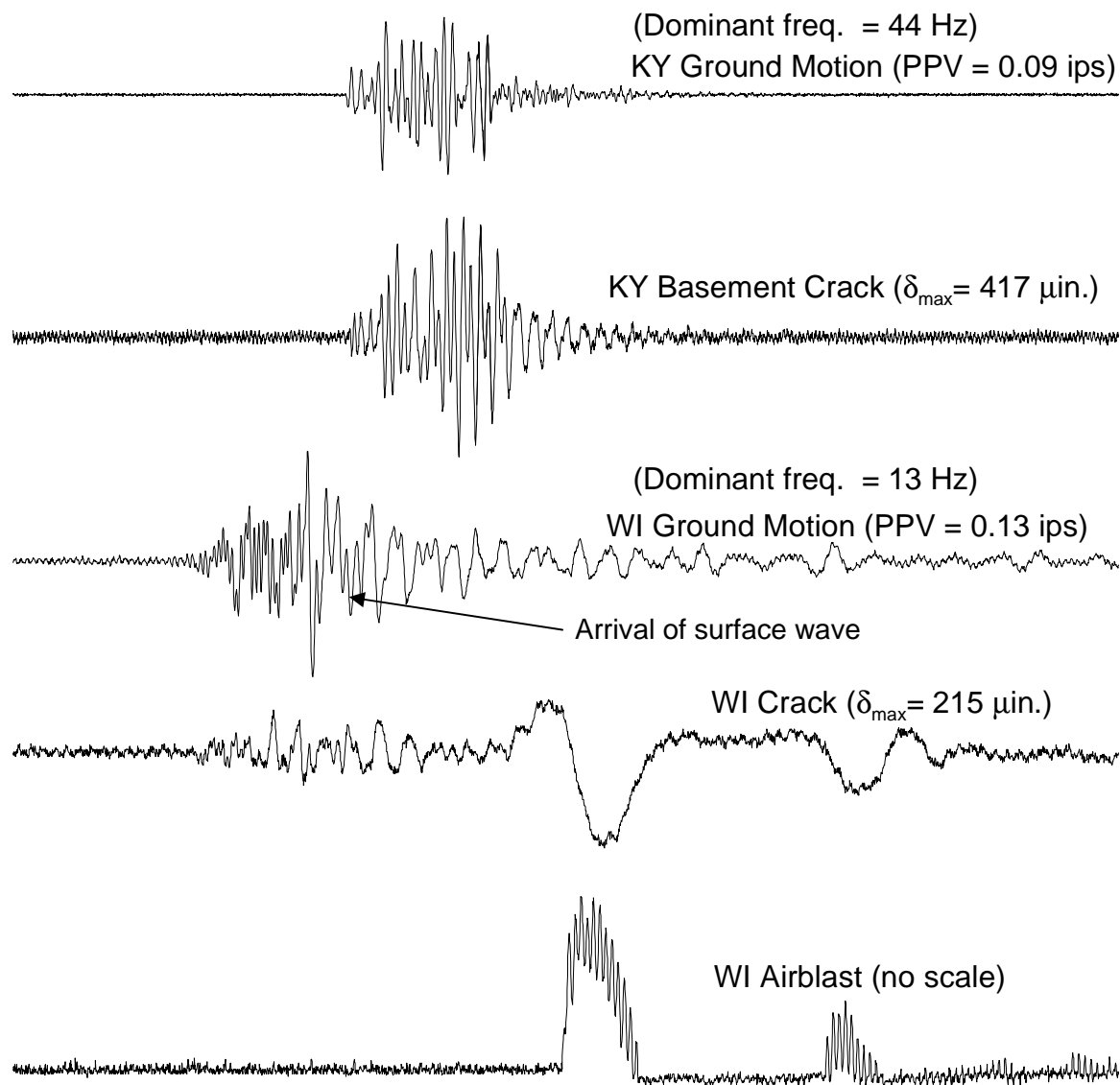
Figure 2.28 Comparison of ground motions and crack response between Kentucky and Wisconsin test structures
