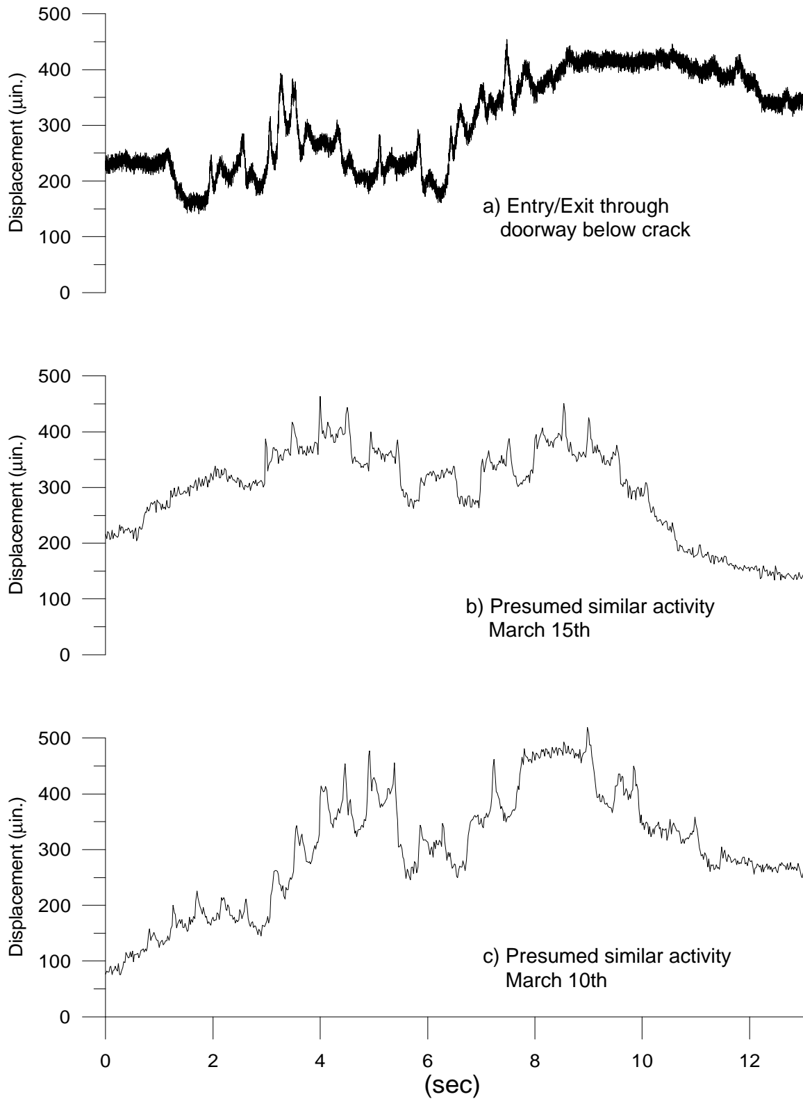
Figure 2.37 Comparison of deliberate and presumed occupant activity bedroom crack response a) induced response during installation of equipment b) & c) presumed response recorded during 50 Hz data collection on respective dates
