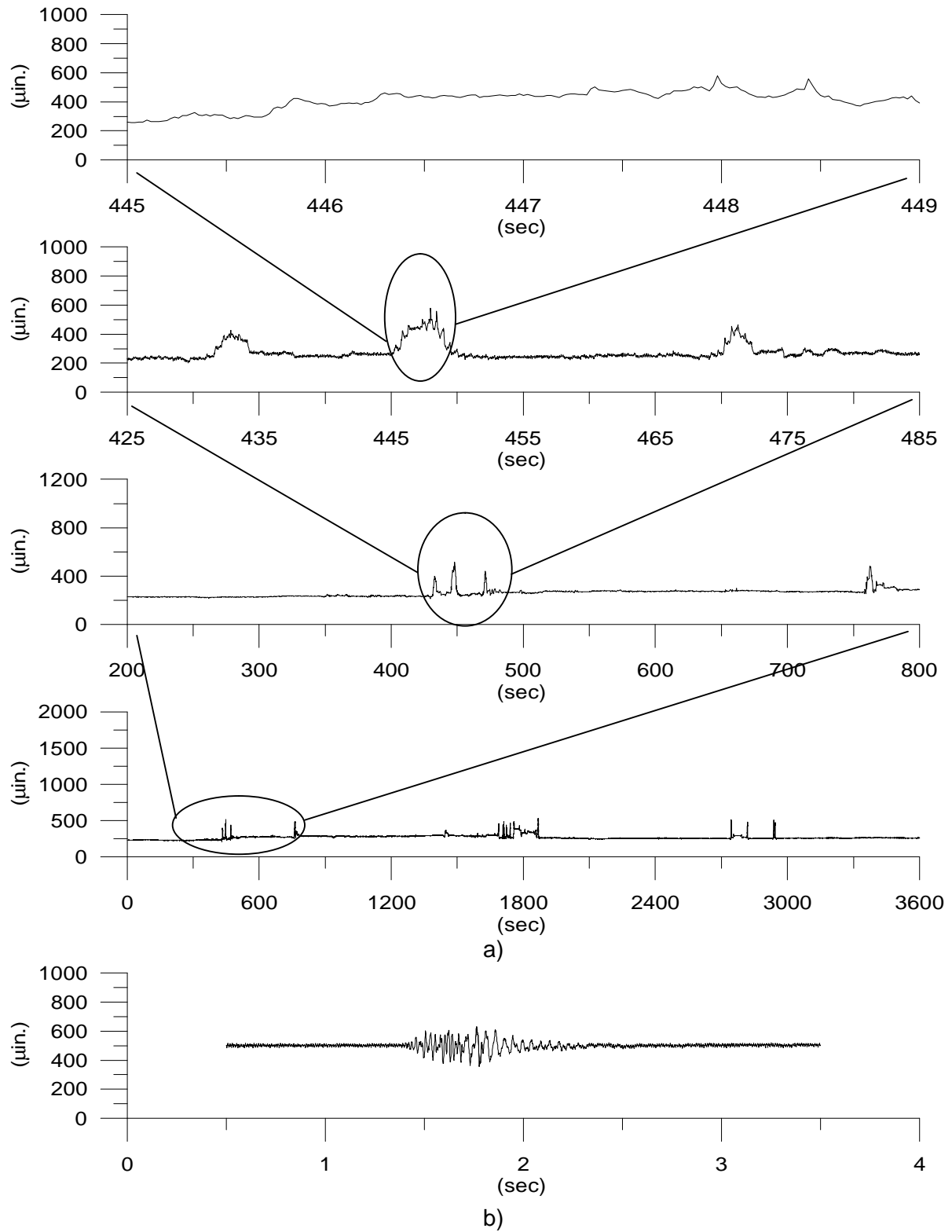
Figure 2.39 Comparison of basement crack displacement for blast and non-blast responses a) 50 Hz data collected during a time period when no blasting occurred (March 9 th ) b) basement crack response to blast (Feb. 8 th )
