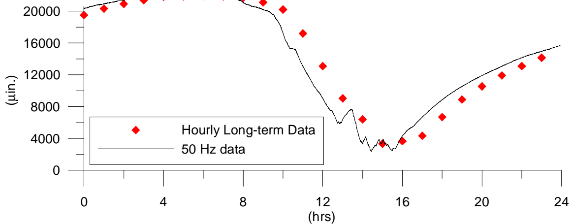
Figure 2.34 Comparison of hourly data and 50 Hz data for the exterior crack (March 4 th )
