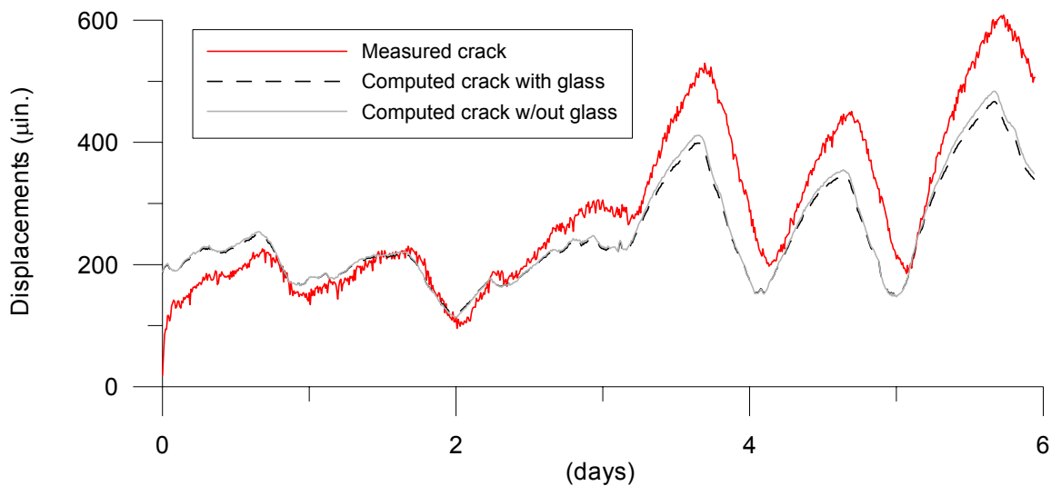
Figure 3.6 Comparison of measured and computed crack displacements for the out-of-plane testing laboratory qualification
