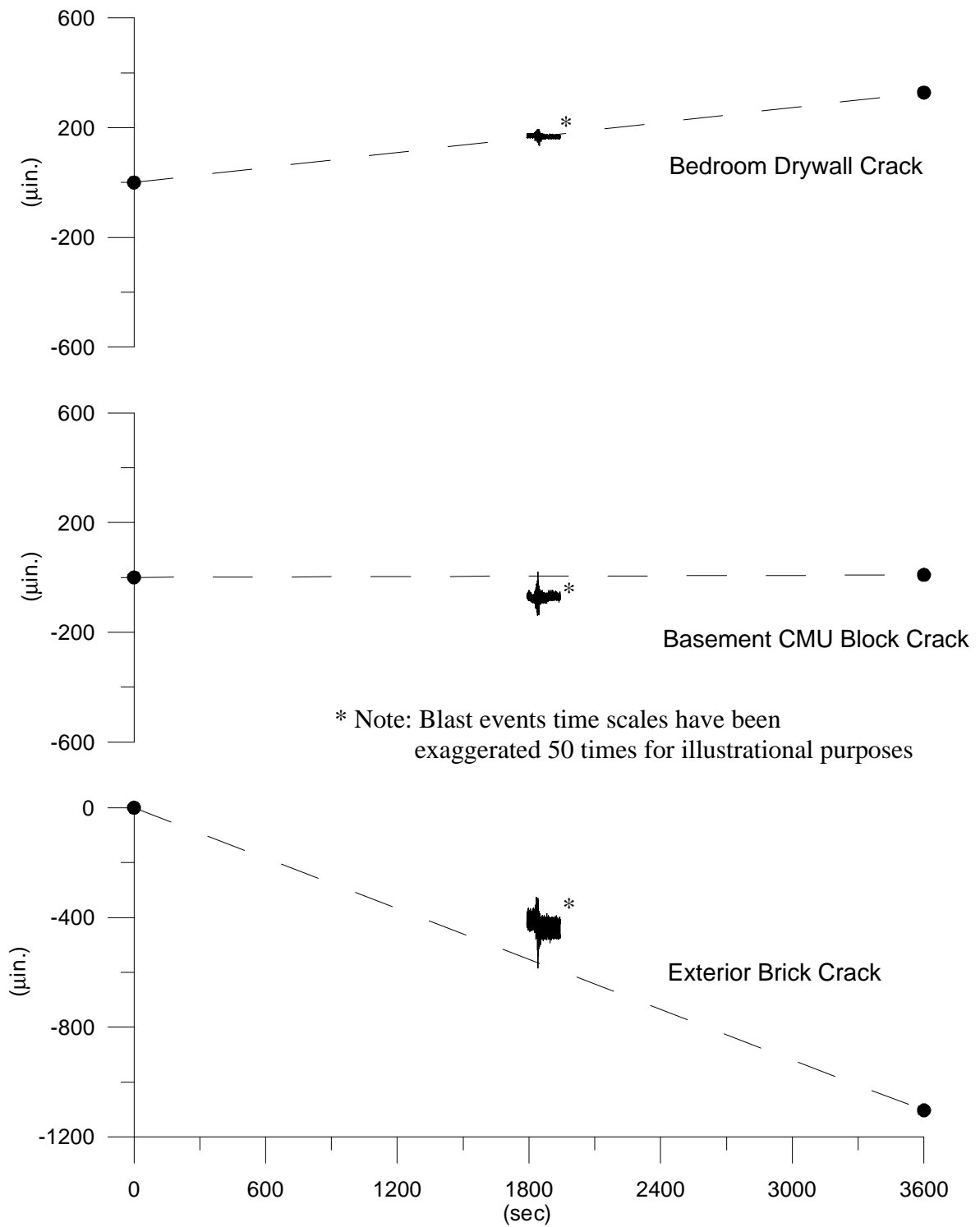
Figure 2.42 Respective crack behavior from blast event compared to crack displacement measured each hour
