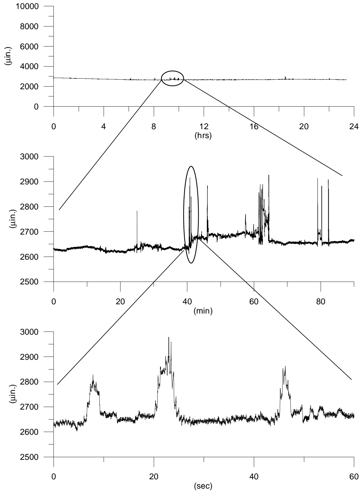
Figure 2.36 Basement crack response during recorded 50 Hz testing
