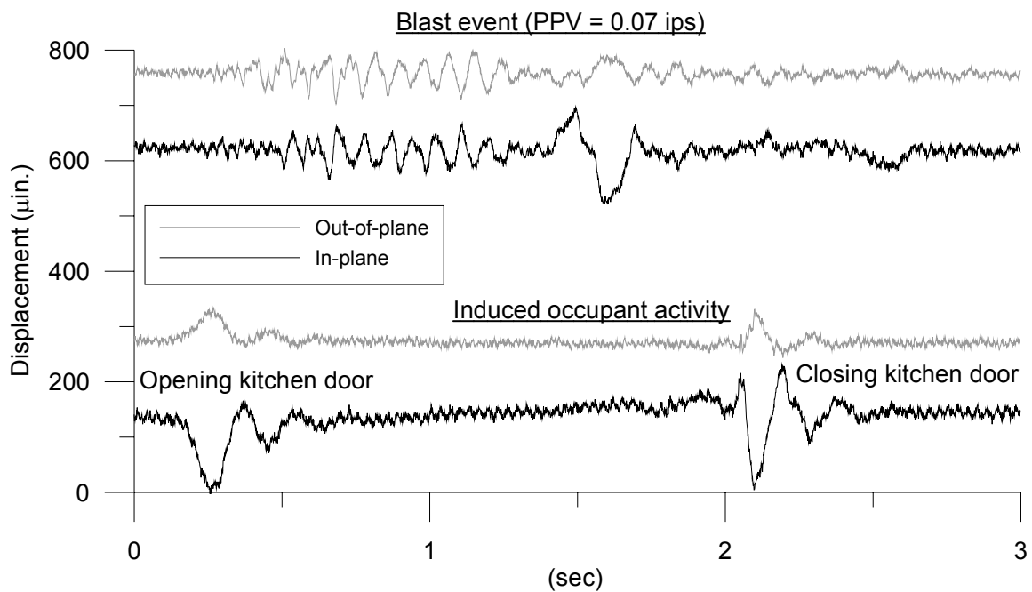
Figure 3.14 Crack response comparison of induced occupant activity (opening and closing of a door) and a blast event (Dec. 28 th PPV = .07 ips) for both directions of displacement measured
