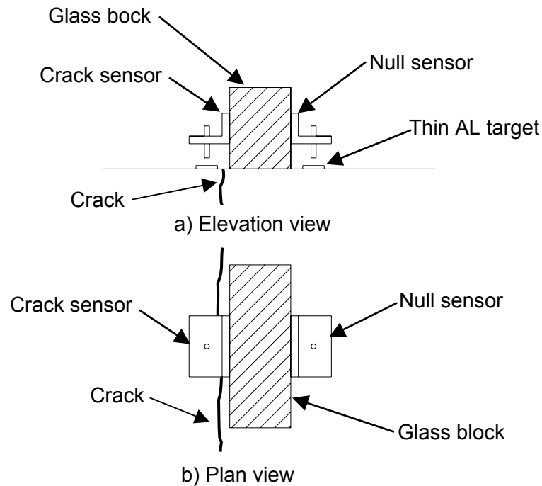
Figure 3.2 Mounting bracket design to measure out-of-plane crack response
