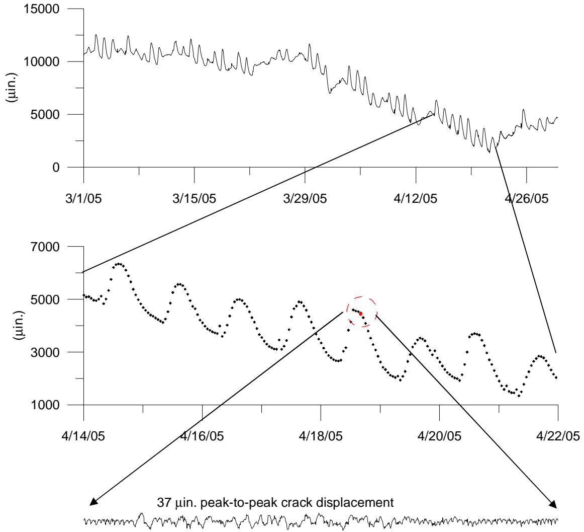
Figure 2.19 Long-term bedroom crack behavior compared to blast event
