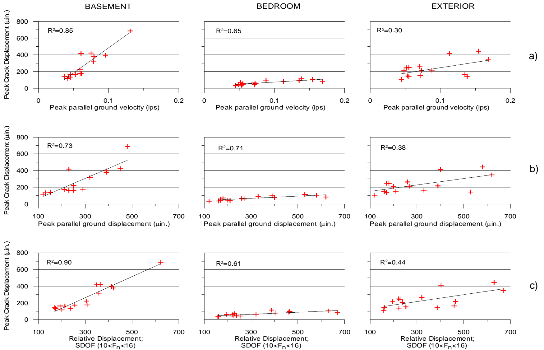
Figure 2.25 Correlations between measured crack displacement and computed displacements and peak ground velocities
