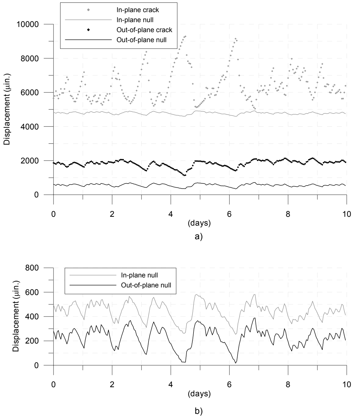
Figure 3.10 Ten day comparison of long-term in-plane and out-of-plane crack behavior a) crack and null behavior for both directions measured b) enlargement of null behavior only for both directions measured
