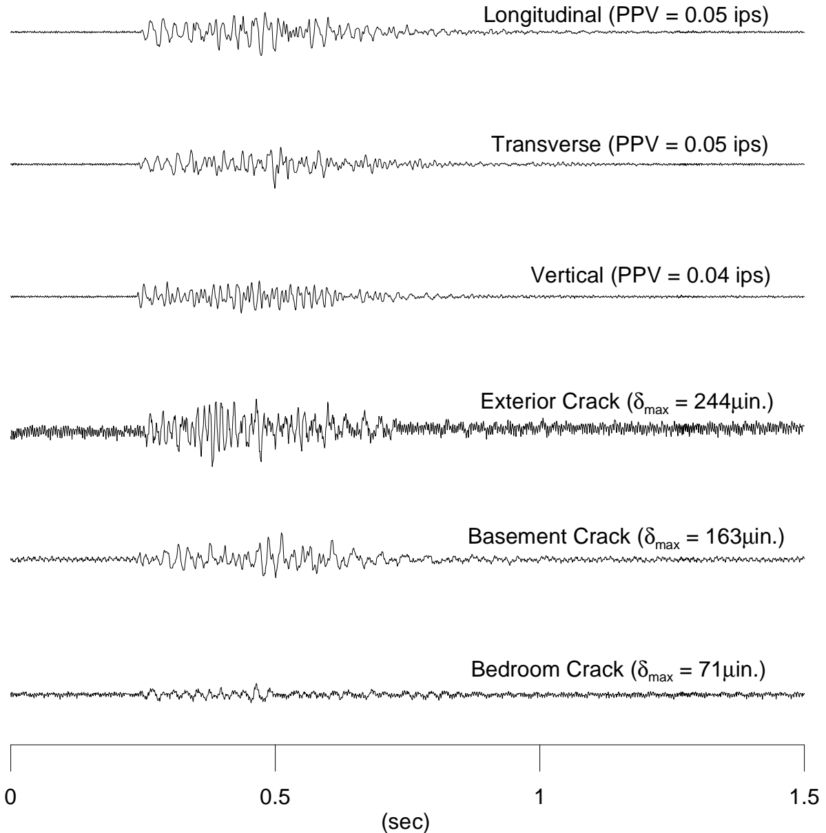
Figure 2.23 Ground motions and crack response for the March 16 th blast
