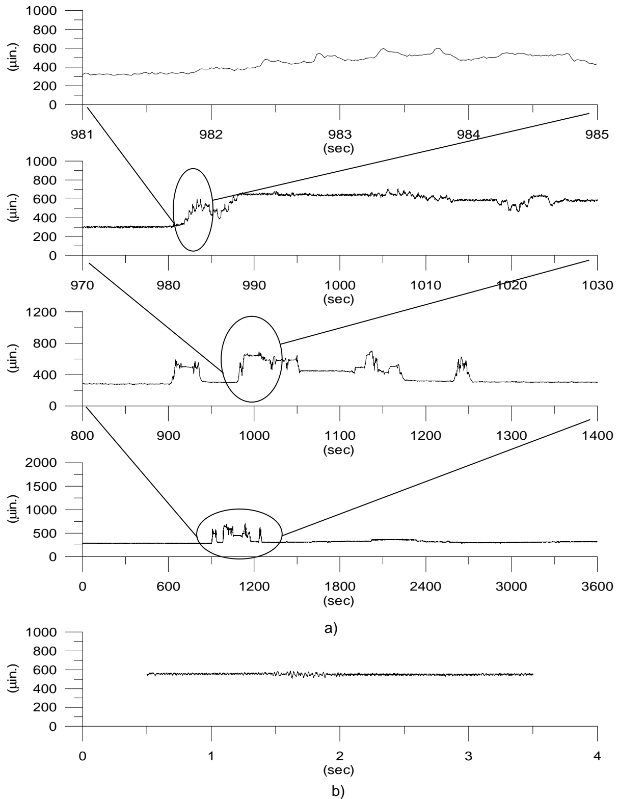
Figure 2.40 Comparison of bedroom crack displacement for blast and non-blast responses a) 50 Hz data collected during a time period when no blasting occurred (March 10 th ) b) bedroom crack response to blast (March 7 th )
