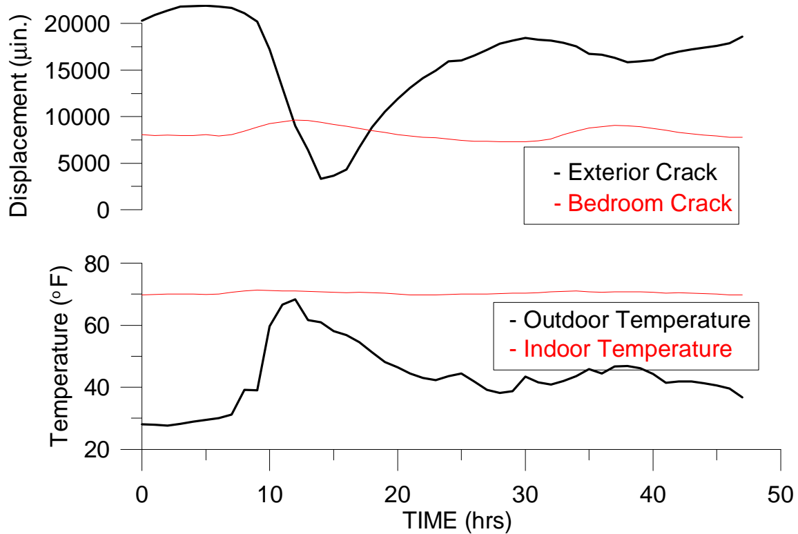
Figure 2.9 Crack responses to temperature over a two-day period
