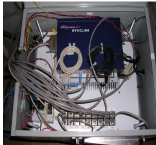
b) Close-up picture of eDAQ and wiring
