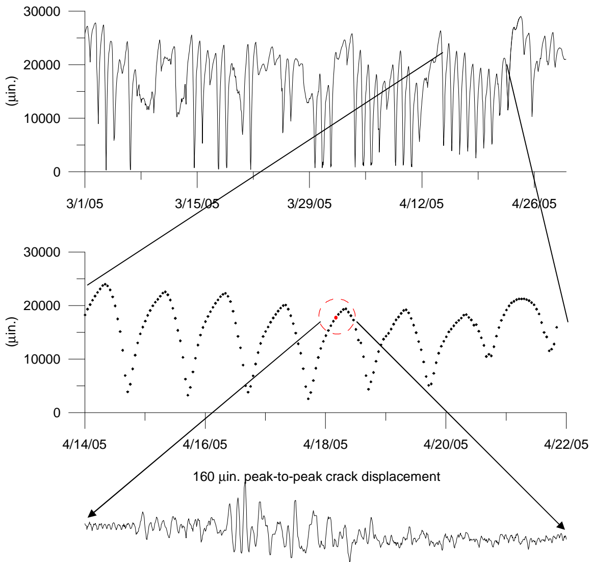
Figure 2.18 Long-term exterior crack behavior compared to blast response
