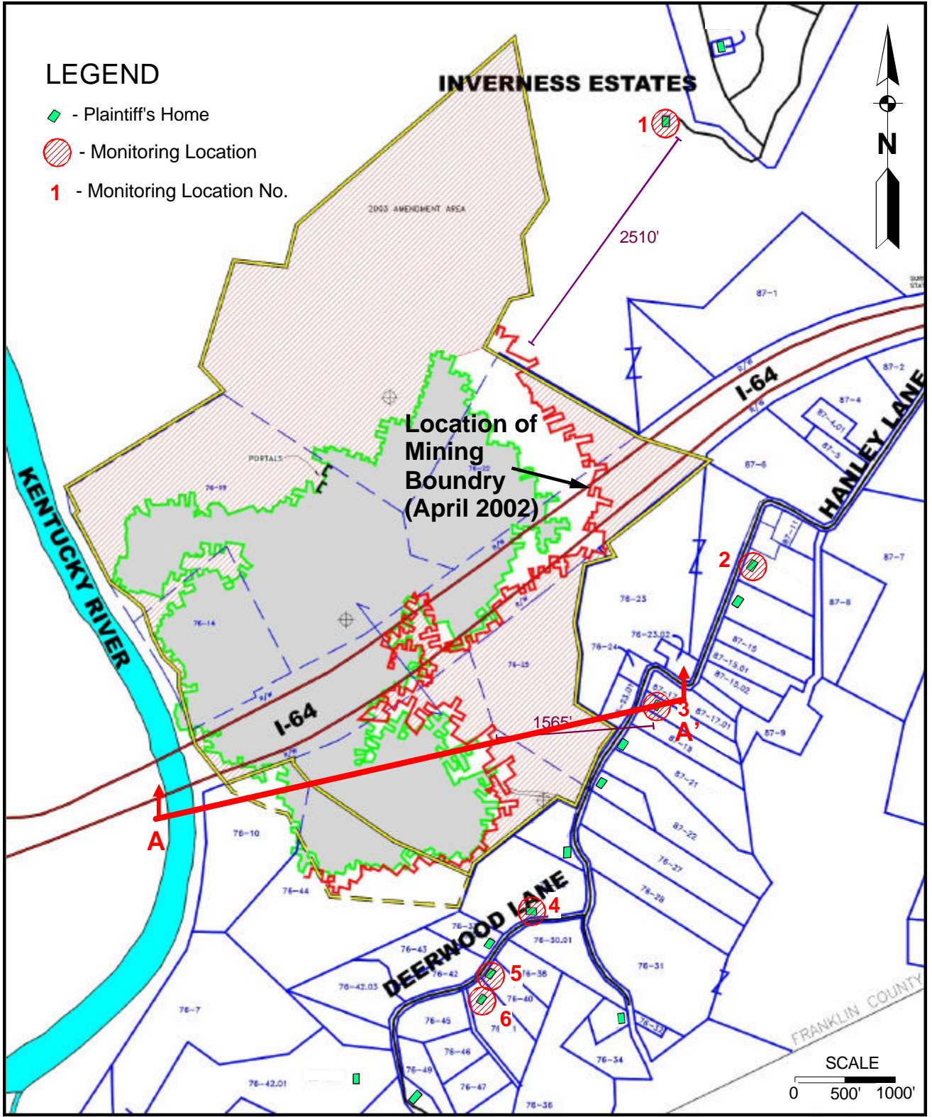
Figure 2.2 Plan view of the extent of the underground mine in relation to the nearby subdivision
