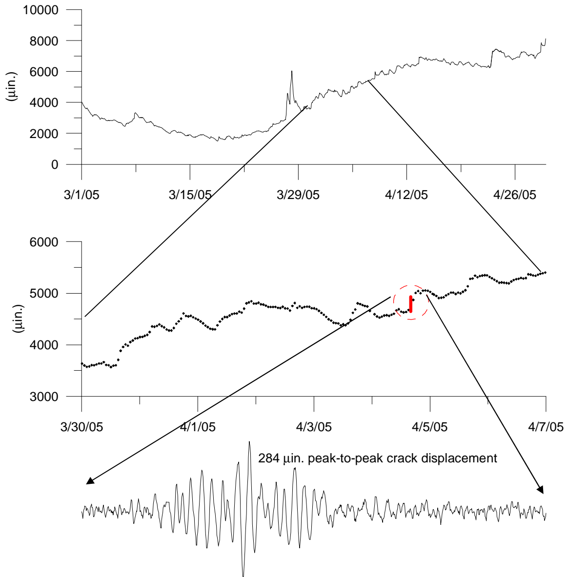
Figure 2.20 Long-term basement crack behavior compared to blast response
