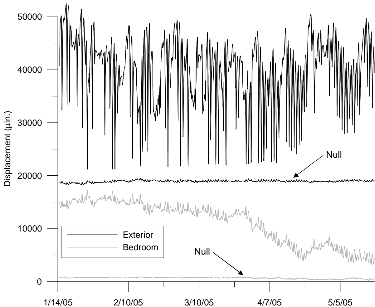
Figure 2.16 Comparison of null sensor displacements to measured crack displacements for the exterior and bedroom cracks
