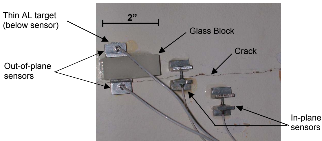
Figure 3.9 Picture of the out-of-plane system installed on a ceiling crack near previously installed in-plane sensors
