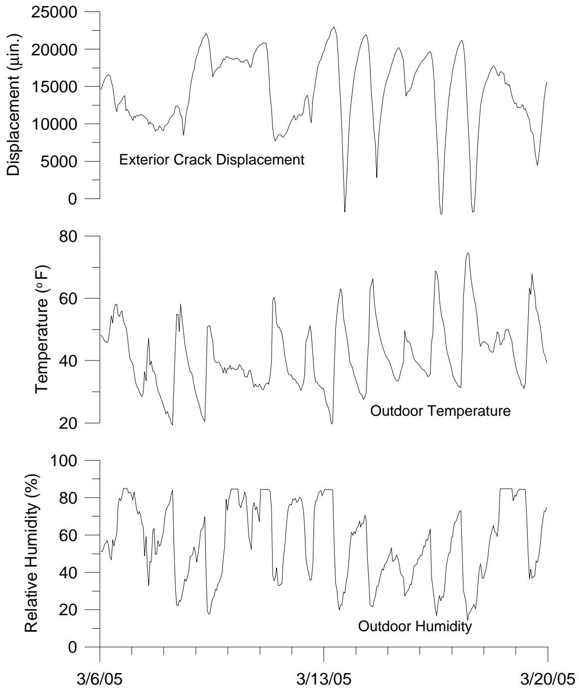
Figure 2.10 Exterior crack response compared with temperature and humidity
