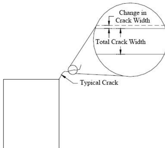
Figure 2.6 Definition of crack displacement (Seibert, 2000)
