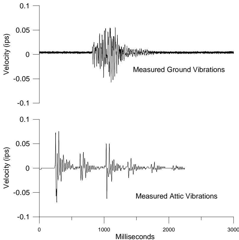
Figure 2.30 Plot of blast ground vibrations and measured attic movements on the same date of March 22 nd
