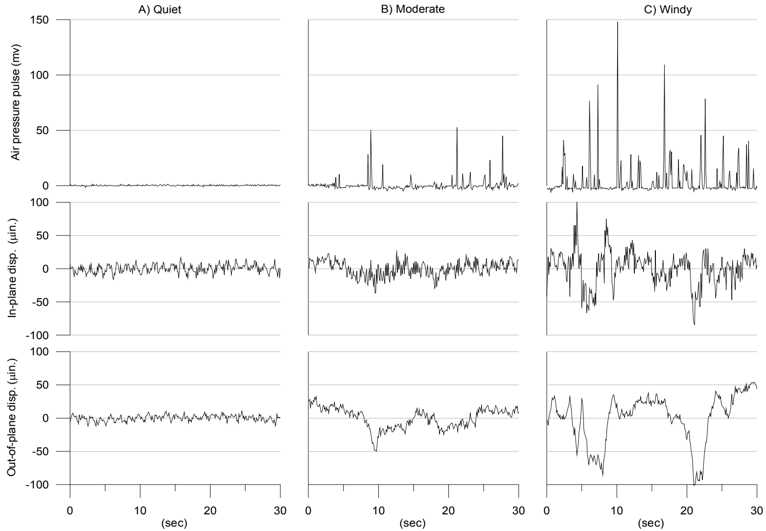
Figure 3.17 Crack behavior during varying degrees of windiness a) a period of low winds b) a period of moderate winds c) a period of high winds
