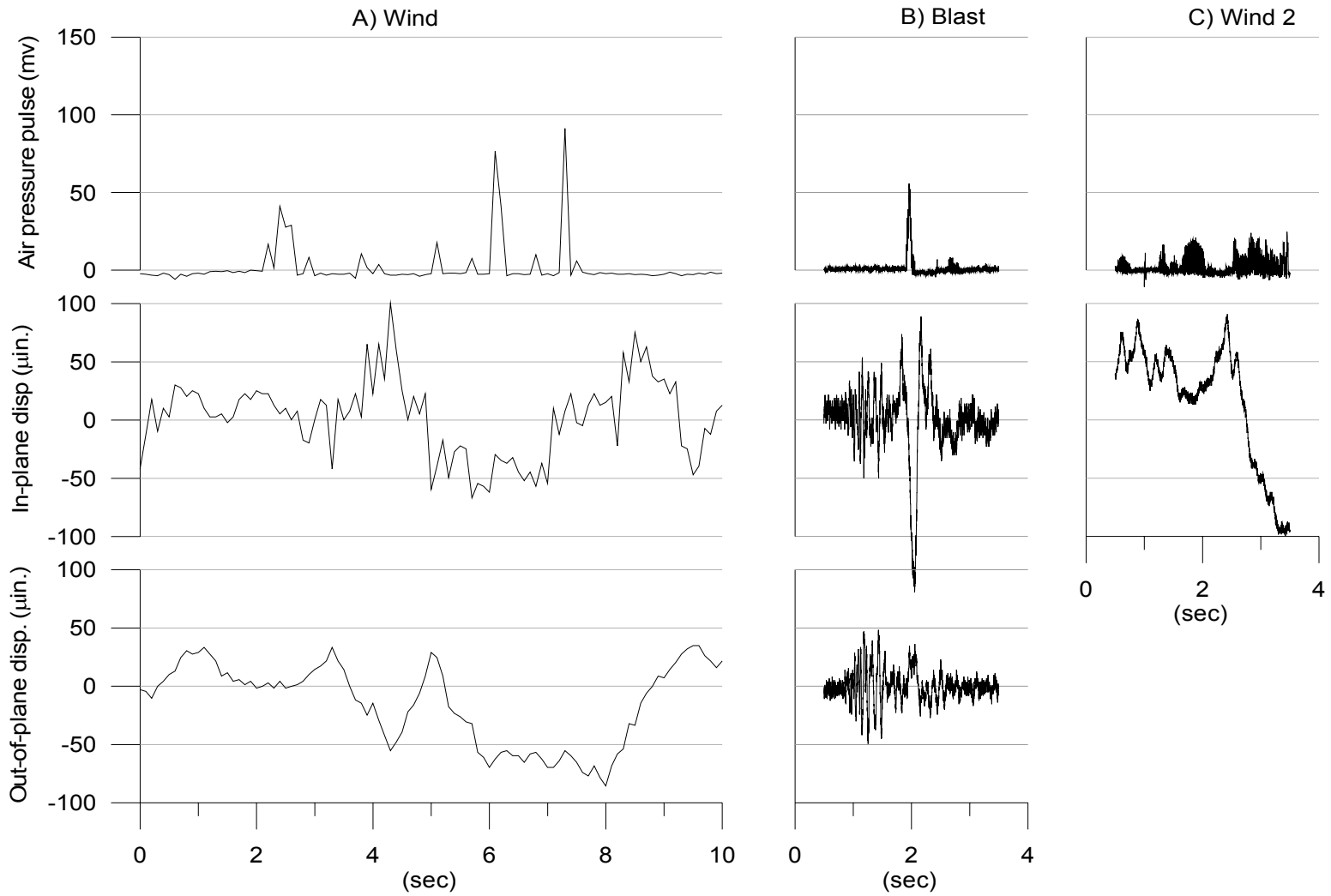
Figure 3.19 Comparison of crack behavior to outdoor winds and a blasting event a) period of high wind b) January 26 th 2006 blast event of PPV = 0.09 ips c) wind induced crack movement obtained on October 30 th 2004
