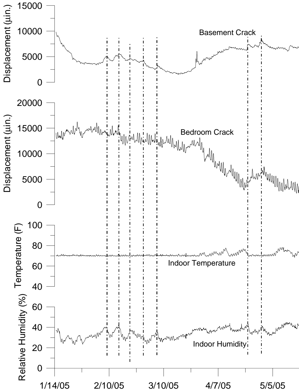
Figure 2.14 Basement and bedroom crack displacement compared to indoor environment conditions
