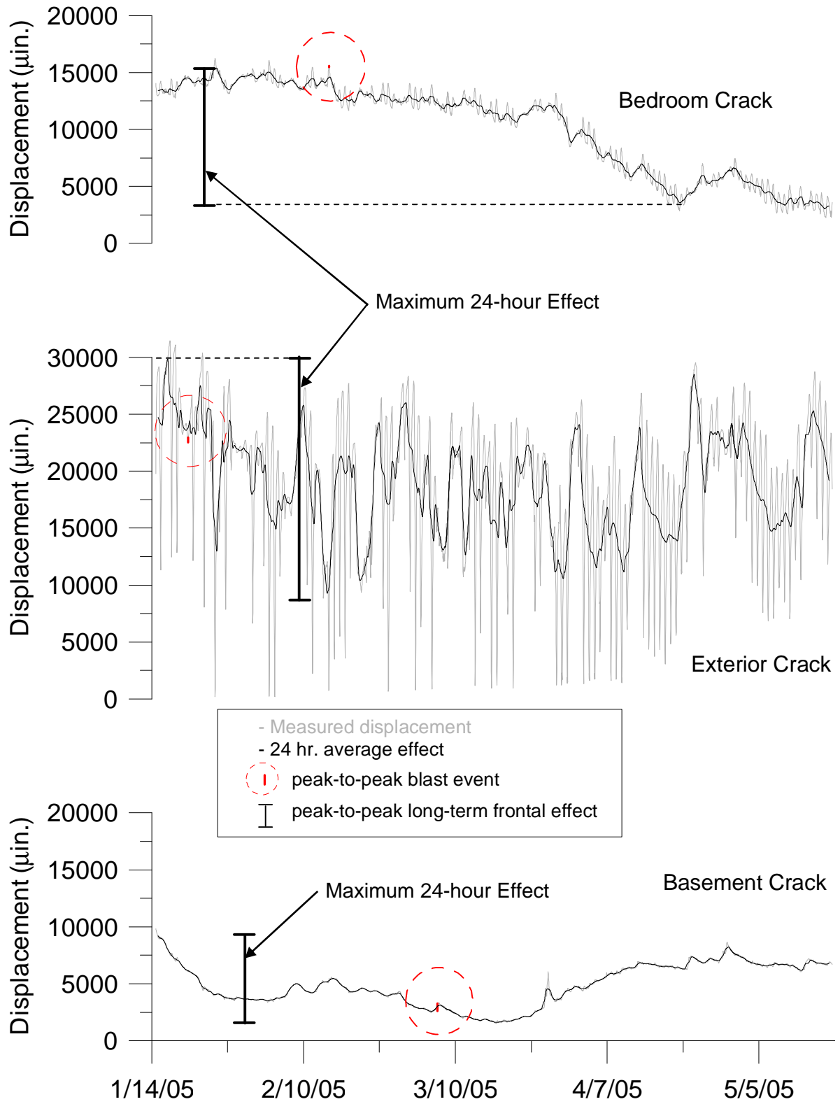
Figure 2.17 Long-term response of all three cracks including to scale the largest corresponding dynamic response
