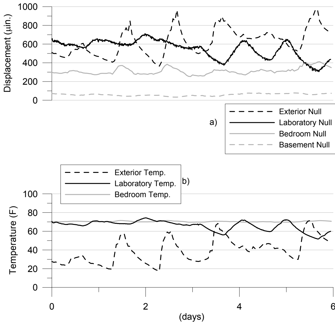
Figure 3.8 Comparison of field null sensors and laboratory null sensors a) null sensors displacements for a six-day period b) temperature conditions affecting null sensors for the corresponding six-day period
