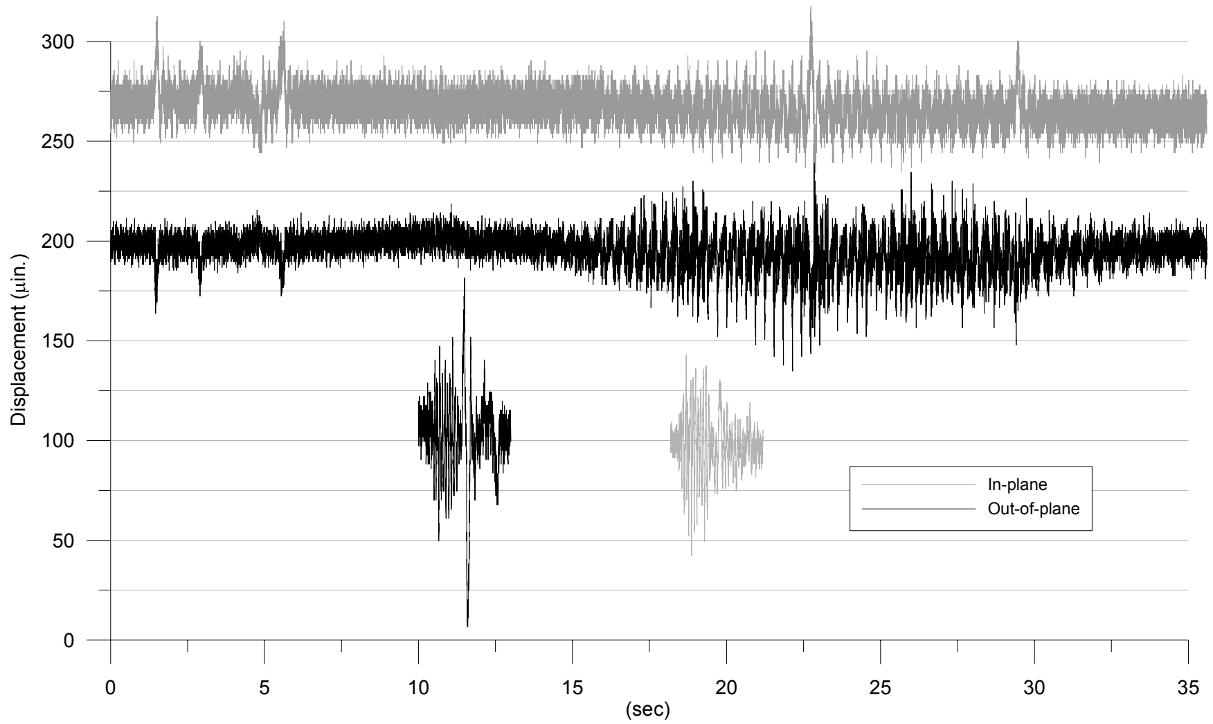
Figure 3.15 Comparison of crack response to ceiling fan and blast event (Dec. 28 th PPV = .07 ips)
