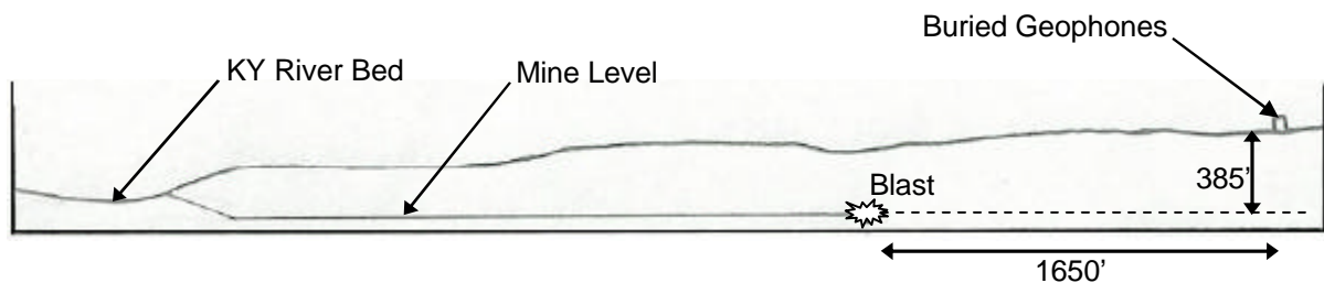
Figure 2.3 Cross-section profile of Frankfort, KY site showing location of residence in relation to blasting. Location of the cross-section is shown above in Figure 2.2
