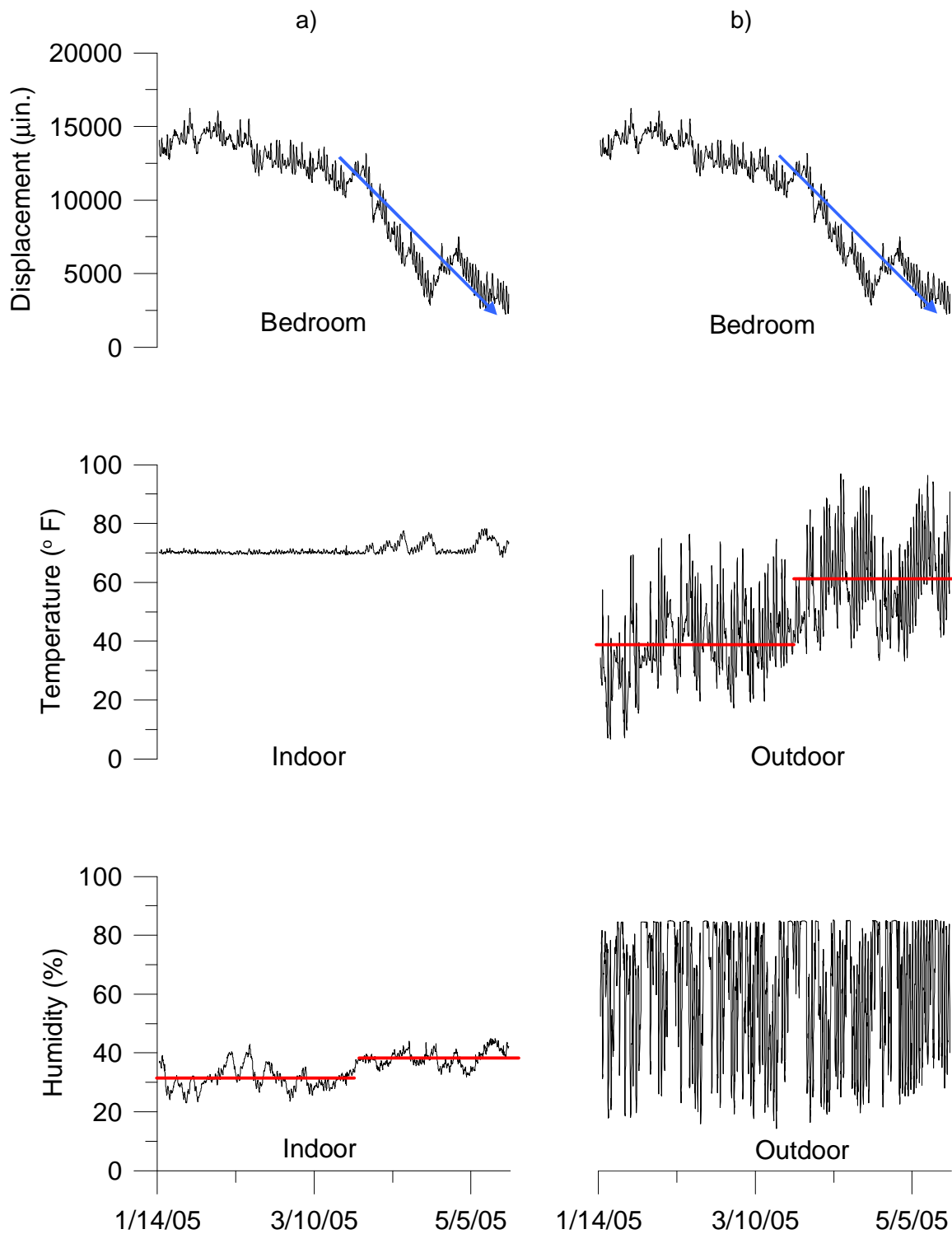
Figure 2.12 Bedroom crack displacement compared to both interior and exterior environmental conditions a) bedroom crack displacement compared to indoor environment conditions b) bedroom crack displacement compared to exterior environment conditions
