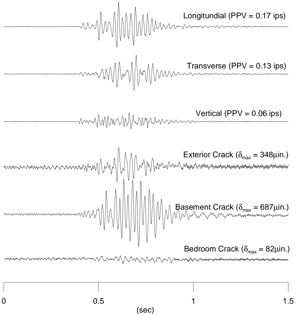
Figure 2.21 Ground motions and crack response for the March 7 th blast
