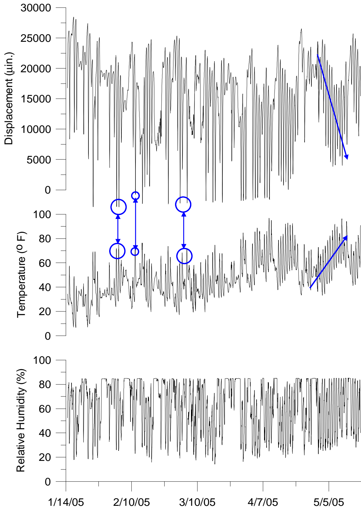
Figure 2.15 Exterior crack displacements compared to outdoor environmental conditions
