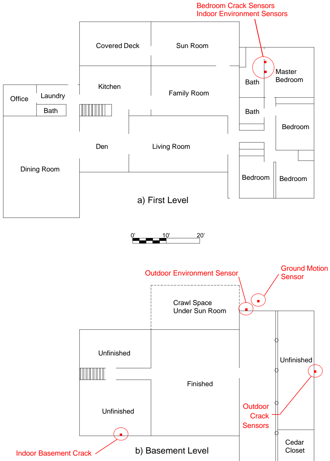
Figure 2.4 Plan view showing locations of sensors; a) bedroom crack in drywall, indoor environment sensors b) indoor basement crack in CMU blocks, outdoor crack in exterior brick, ground motion sensors, and outdoor environment sensors
