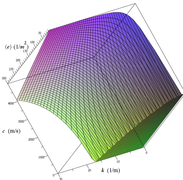
Figure 4: Phase velocity c —wave number k —damage factor \langle e \rangle surface
