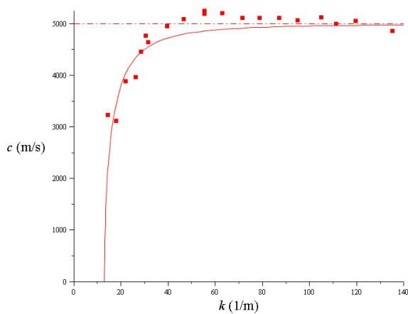
Figure 5: Dispersion curve of the thin Aluminium rod. Dash dot line: without random damage \langle e \rangle = 0 m -2 ; Solid line: with random damage \langle e \rangle = 170 m -2 ; Solid box points: experiment by Kinra et al (Kinra and Rousseau, 1987) with volume fraction of random inclusions as 15%.
