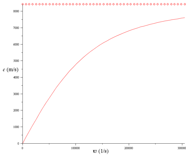
Figure 11: Dispersion curve of the thin silicon crystal rod. Solid line: with random damage, \langle e \rangle is 300 \text{ m}^{-2} ; Diamond point line: without random damage, \langle e \rangle = 0 \text{ m}^{-2} .
